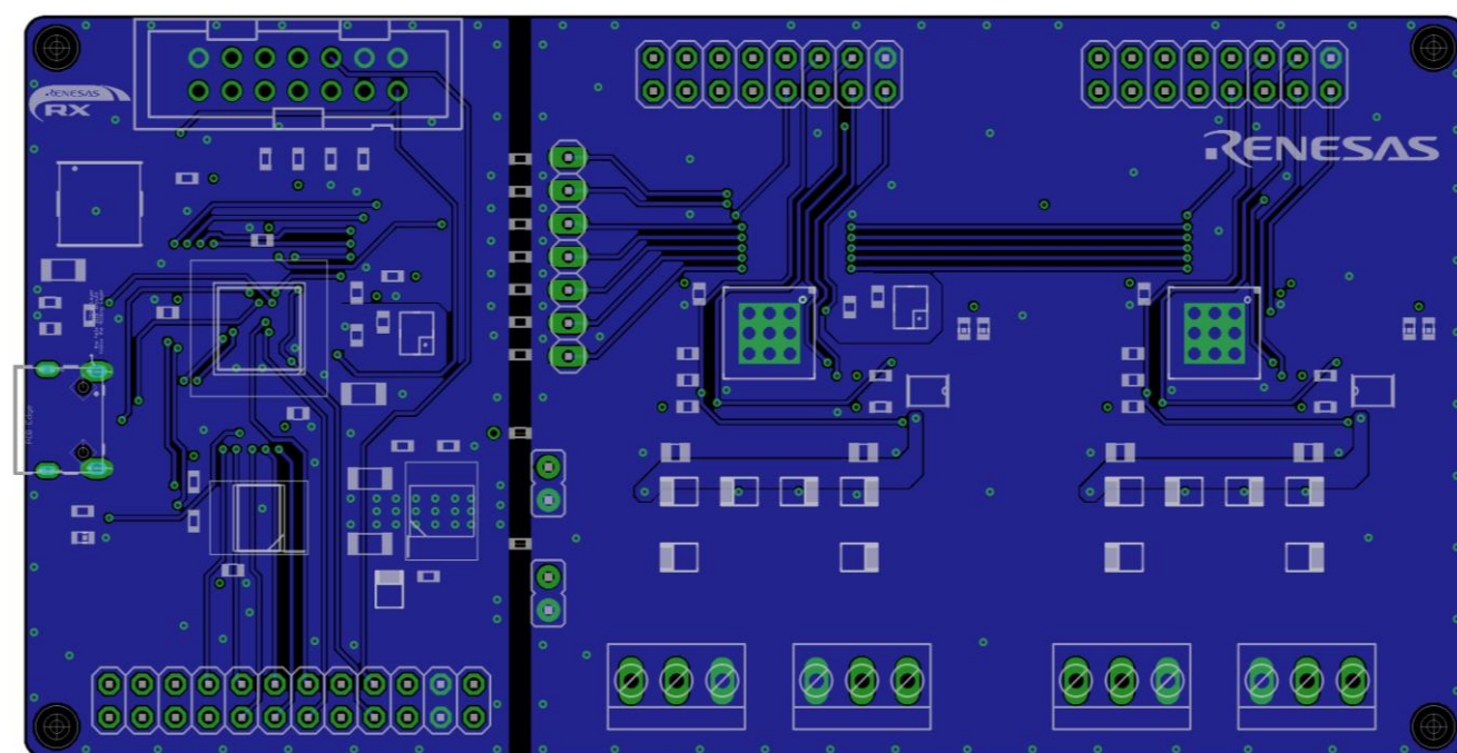
Figure 10. Bottom Layer
