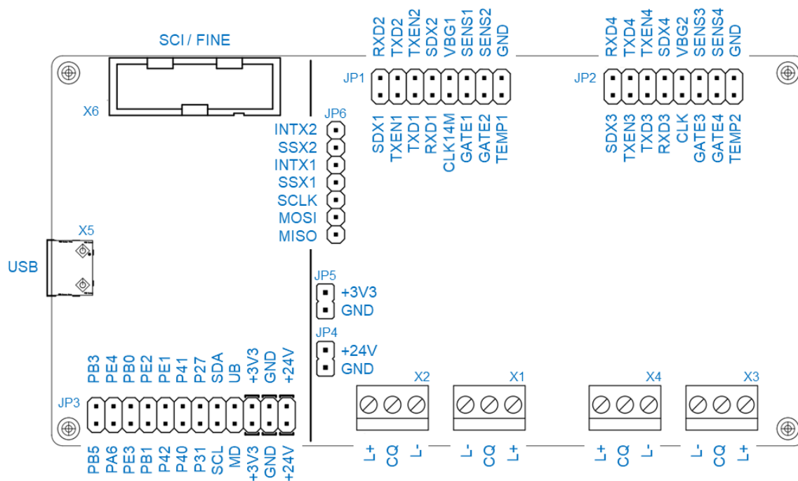
Figure 4. Connectors
