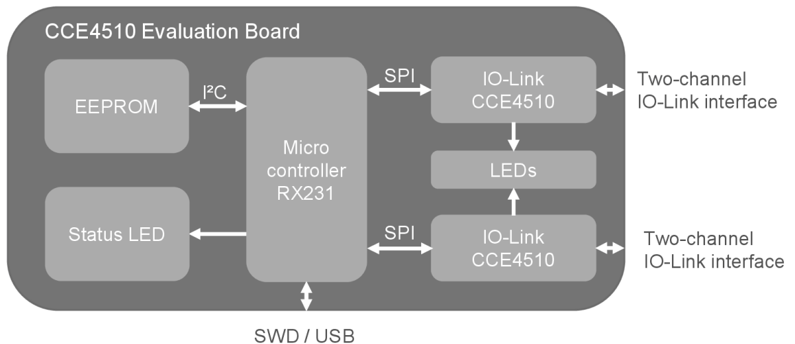
Figure 2. System Diagram
