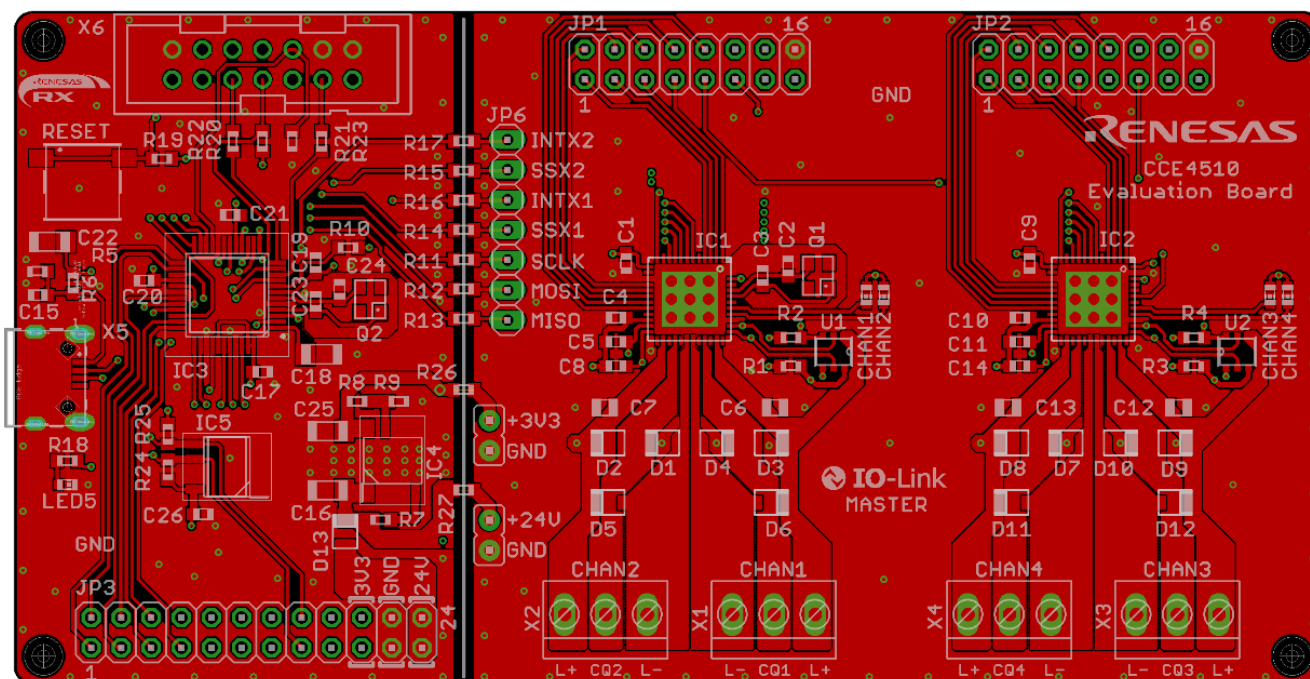
Figure 7. Top Layer
