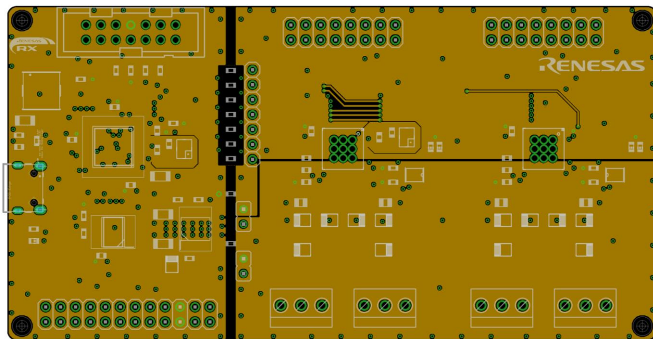
Figure 9. Third Layer (Supply)
