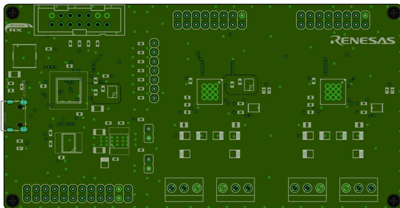
Figure 8. Second Layer (GND)
