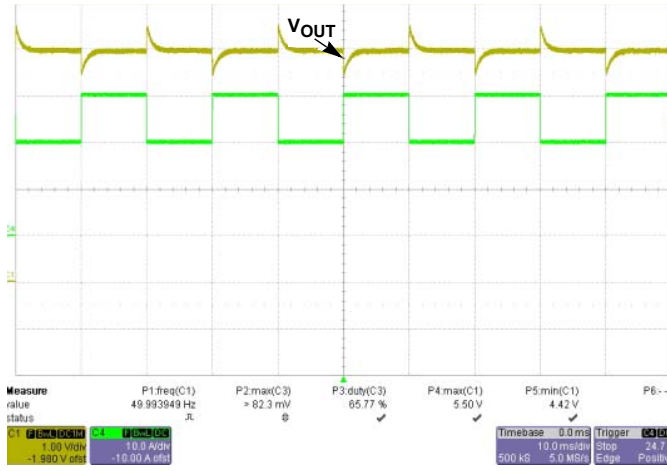
FIGURE 56. ±530mV @ 75%-50%-75% LOAD, 0.2A/μs, V IN = 36V (YELLOW = V O , GREEN = I O )
