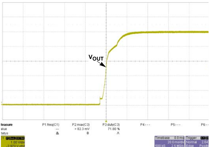
FIGURE 34. RECOVERY @ 33V, I_O = 40A
