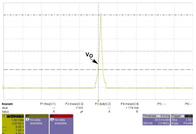
FIGURE 40. OVP @ V_{IN} = 75V, I_O = 40A
