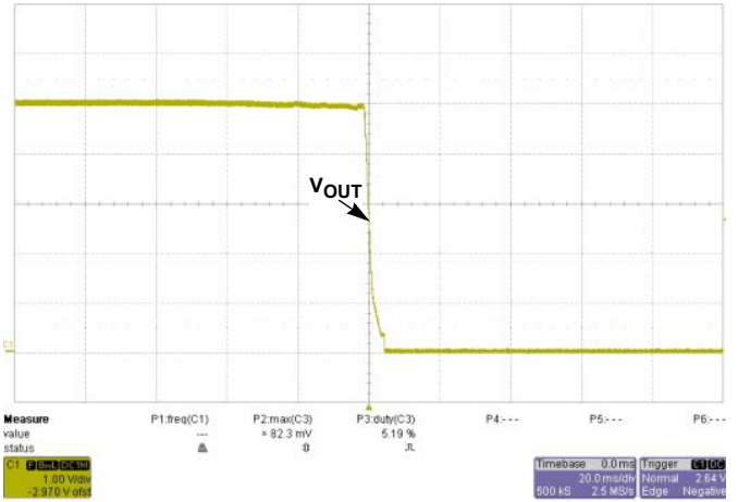
FIGURE 30. SHUT-DOWN AT V_{IN} = 75V @ I_O = 40A
