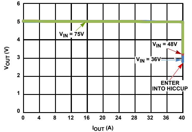
FIGURE 44. OCP CHARACTERISTICS
