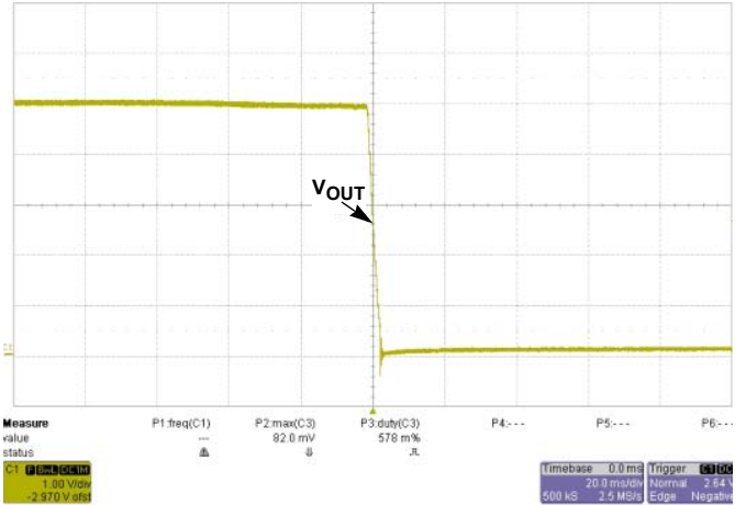
FIGURE 12. SHUT-DOWN AT V_{IN} = 48V @ I_O = 0A
