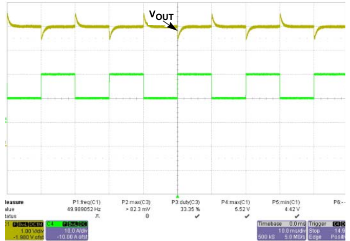
FIGURE 59. ±540mV @ 25%-50%-25% LOAD, 0.2A/μs, V IN = 48V (YELLOW = V O , GREEN = I O )
