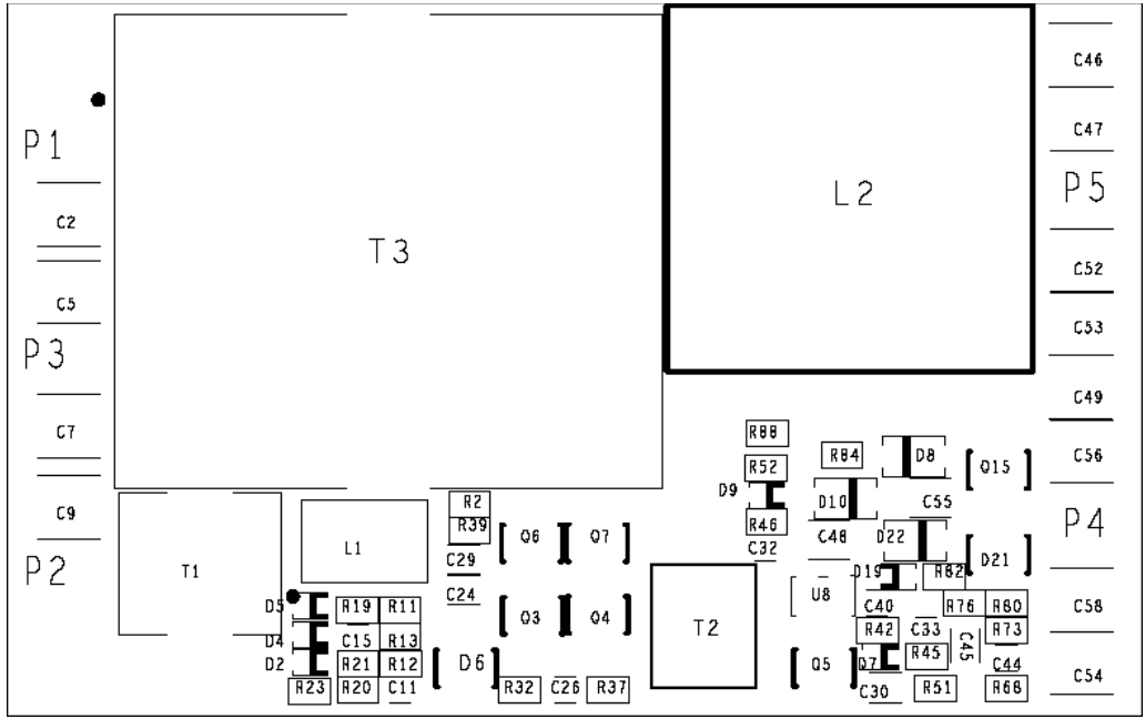
FIGURE 4. ISL6726EVAL1Z TOP VIEW
