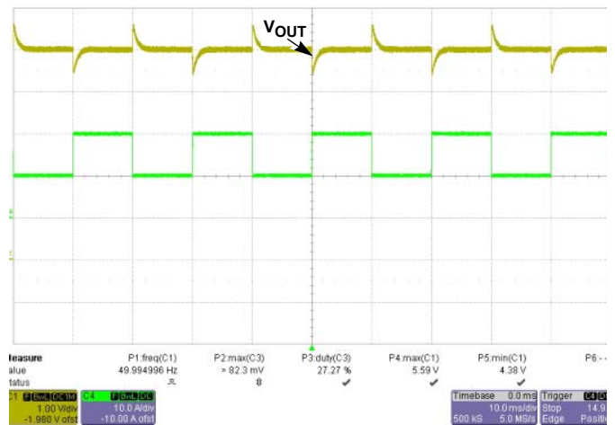
FIGURE 61. ±600mV @ 25%-50%-25% LOAD, 0.2A/μs, V IN = 75V (YELLOW = V O , GREEN = I O )
