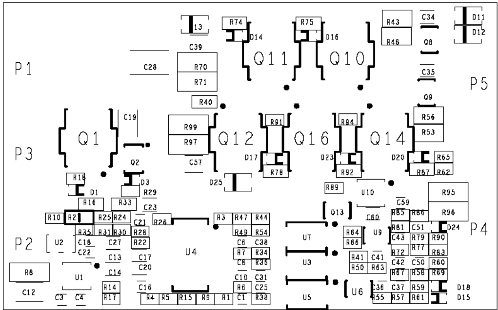
FIGURE 5. ISL6726EVAL1Z BOTTOM VIEW
