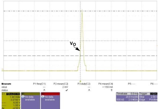
FIGURE 36. OVP @ V_{IN} = 36V, I_O = 40A
