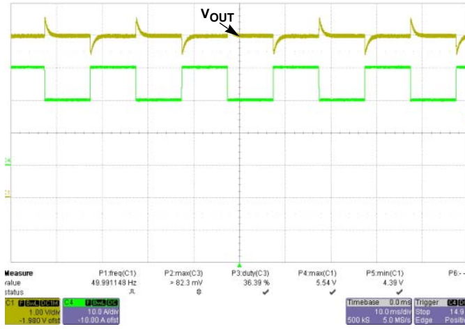
FIGURE 58. ±540mV @ 75%-50%-75% LOAD, 0.2A/μs, V IN = 48V (YELLOW = V O , GREEN = I O )
