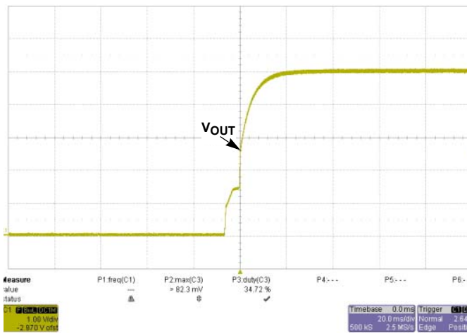
FIGURE 15. START-UP (30ms) AT V_{IN} = 75V @ I_O = 0A
