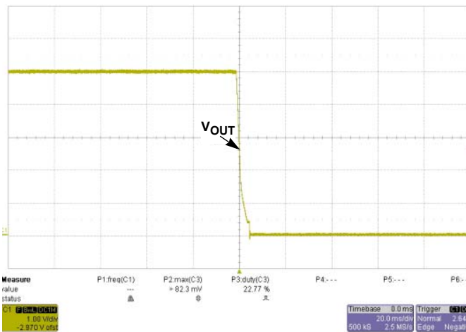
FIGURE 33. UVP @ 30.9V, I_O = 40A
