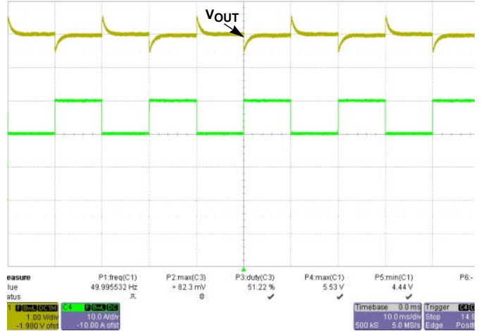
FIGURE 57. ±530mV @ 25%-50%-25% LOAD, 0.2A/μs, V IN = 36V (YELLOW = V O , GREEN = I O )
