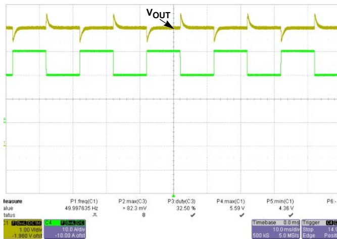
FIGURE 60. ±600mV @ 75%-50%-75% LOAD, 0.2A/μs, V IN = 75V (YELLOW = V O , GREEN = I O )
