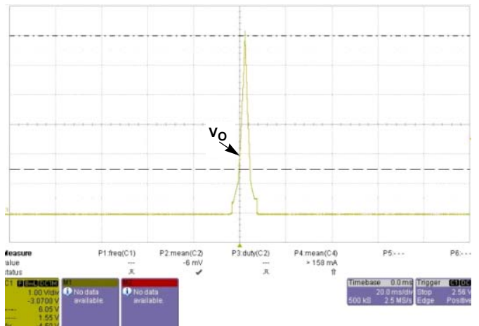
FIGURE 38. OVP @ V_{IN} = 48V, I_O = 40A
