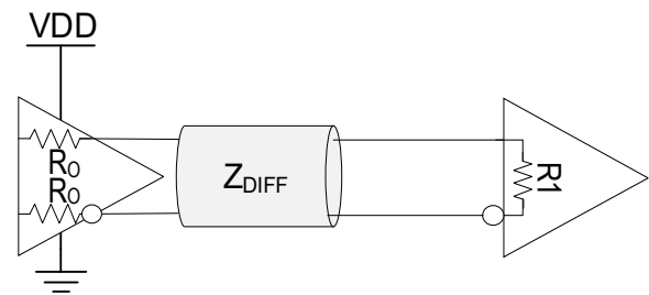
Figure 16. LVDS Output Termination
