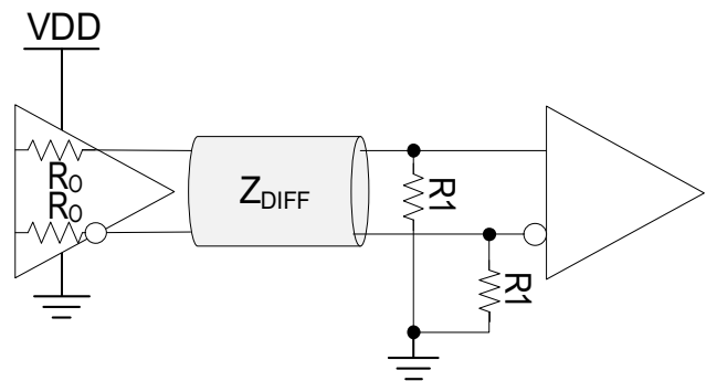
Figure 17. HCSL Output Termination
