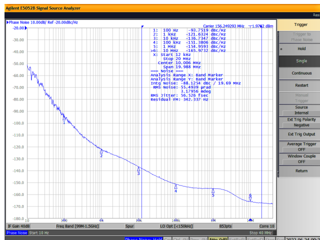
Figure 9. 3.3V HCSSL, 156.25MHz
