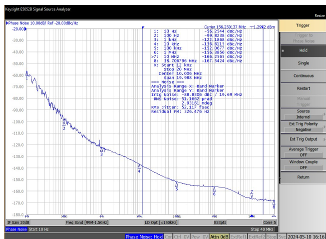
Figure 12. 1.8V HCSSL, 156.25MHz
