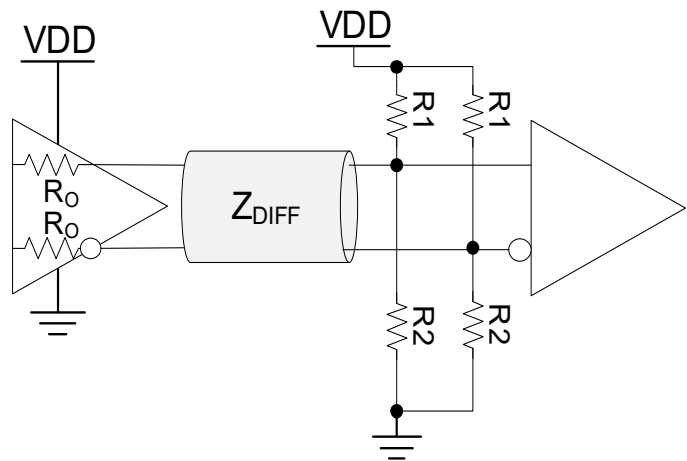
Figure 15. LVPECL Output Termination
