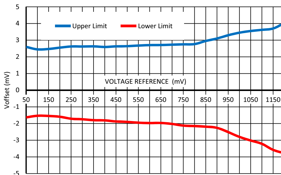
Figure 27. Typical Input Voltage Offset vs. Voltage Reference at room temperature, LBW Mode – Disable, V_{hys}=0 mV, V_{DD}=(1.7 - 5.5) V.
