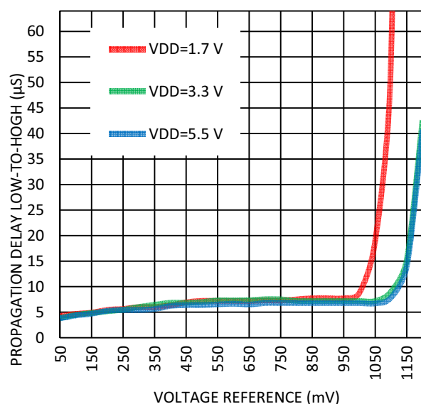
Figure 33. Maximum Propagation Delay Low-to-High vs. Voltage Reference at Room Temperature, V_{od} = 2 \text{ mV} .
