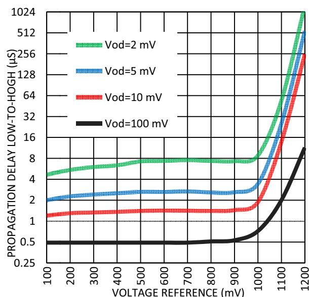
Figure 34. Maximum Propagation Delay Low-to-High vs. Voltage Reference at Room Temperature, V_{DD} = (1.71 - 1.89) \text{ V} .
