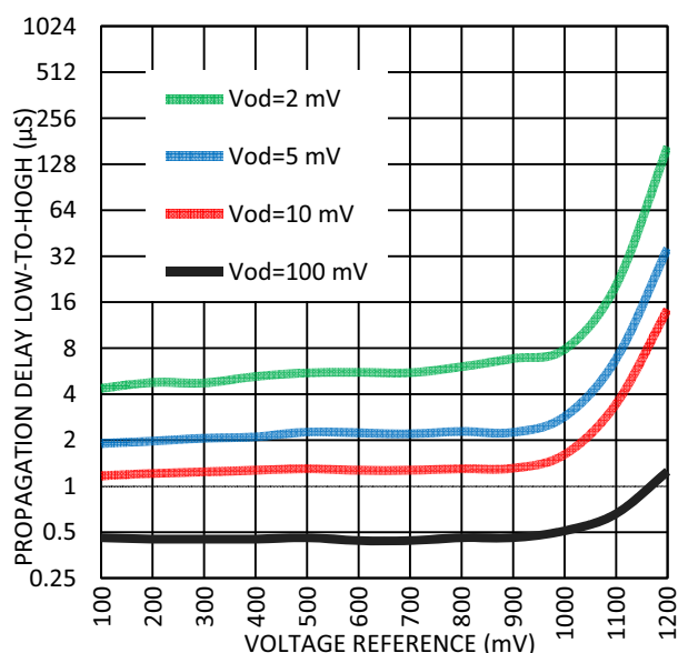
Figure 36. Maximum Propagation Delay High-to-Low vs. Voltage Reference at Room Temperature, V_{DD} = (1.71 - 1.89) \text{ V} .
