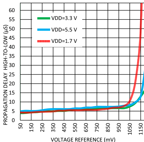
Figure 35. Maximum Propagation Delay High-to-Low vs. Voltage Reference at Room Temperature, V_{od} = 2 \text{ mV} .
