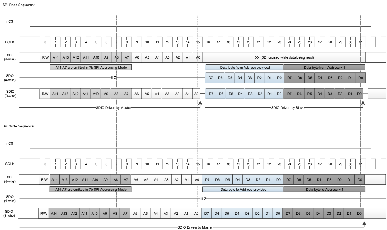
Figure 21. SPI Sequencing
