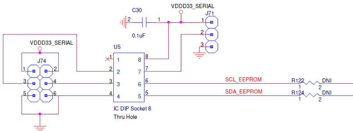
Figure 22. EEPROM Schematic
