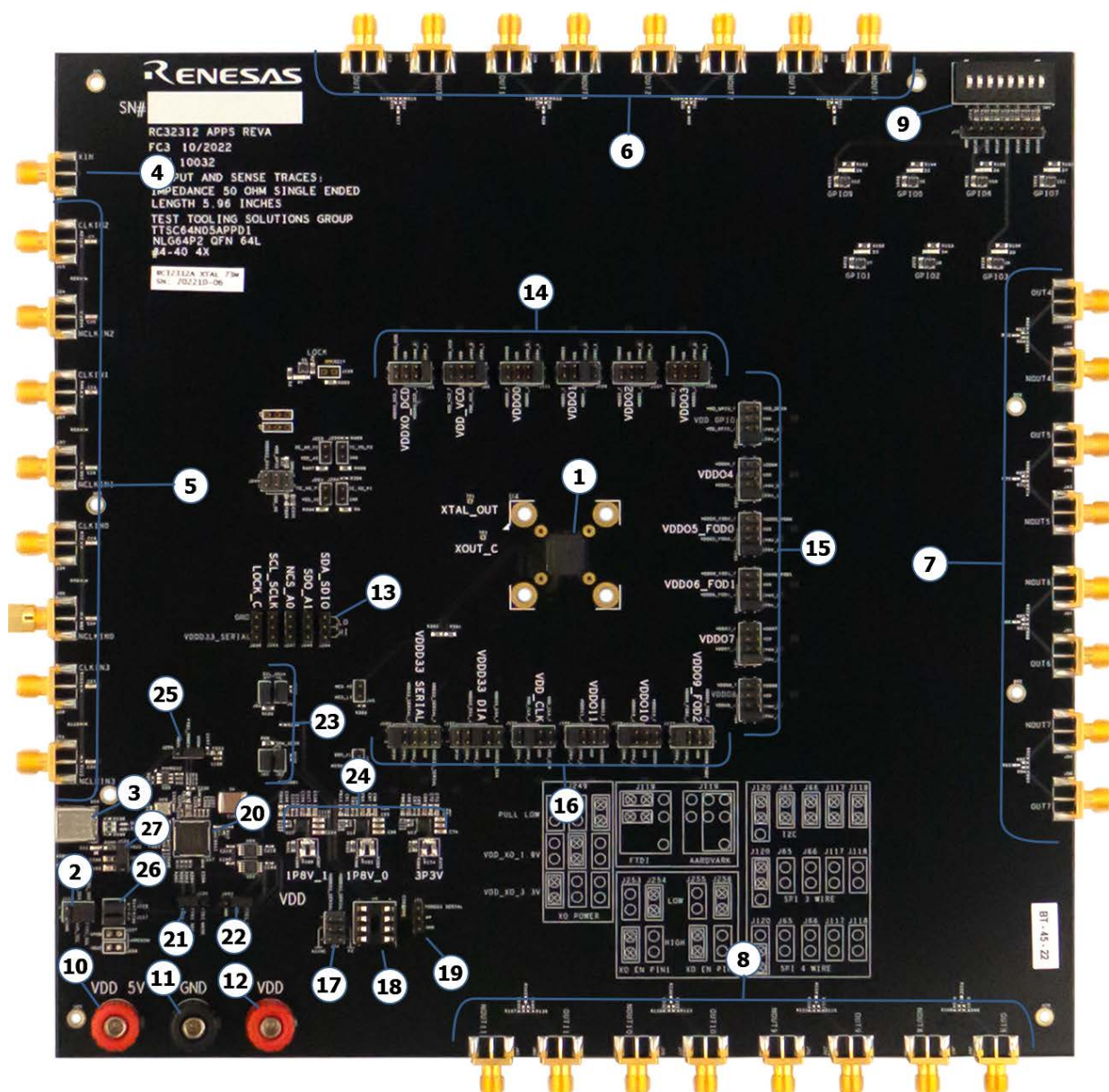
Figure 2. Evaluation Board
