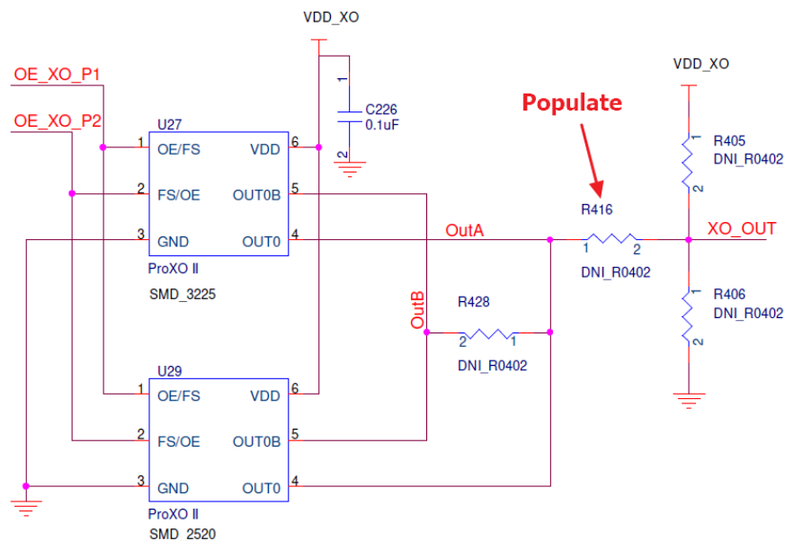
Figure 12. XO Schematic
