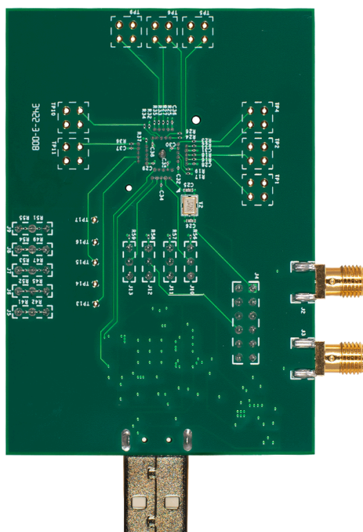
Figure 15. RC21214/RC21213 Evaluation Board (Bottom)
