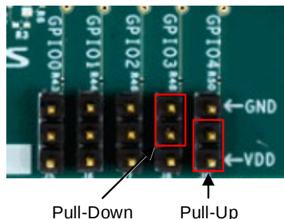
Figure 6. GPIO Jumper Settings
