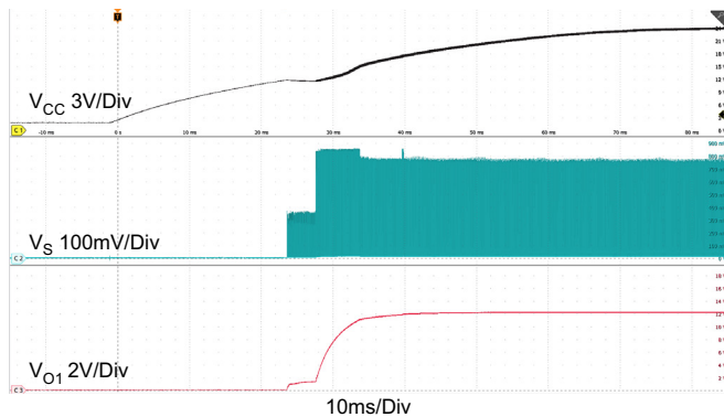
Figure 14. Startup
