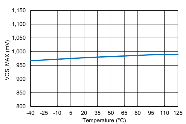
Figure 7. Maximum Current Sensing Threshold vs Temperature
