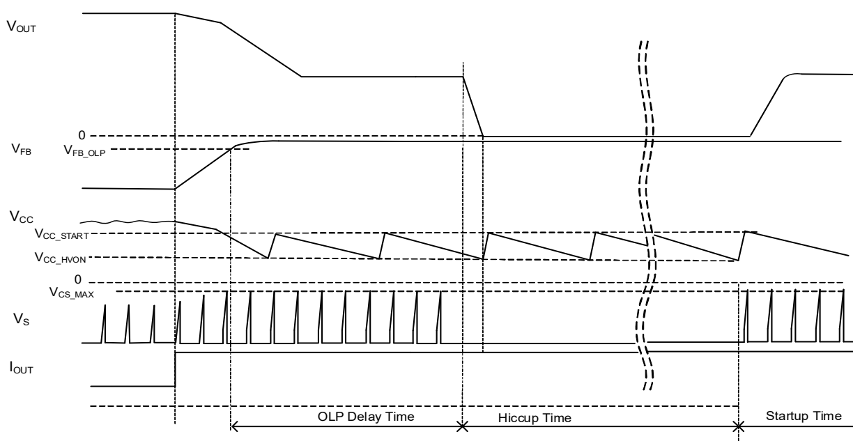
Figure 25. Overload Protection Diagram
