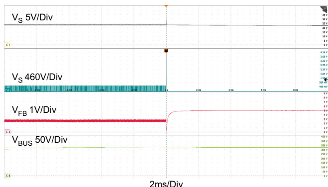
Figure 20. Short-Winding Protection
