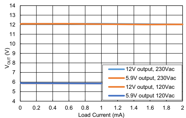
Figure 13. Load Regulation
