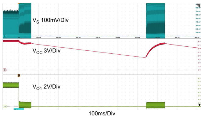
Figure 18. Short-Circuit Protection
