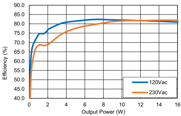
Figure 12. Efficiency
