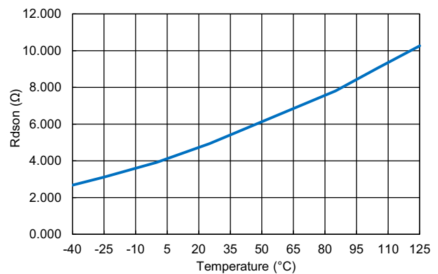
Figure 5. r_{\text{DS(ON)}} vs Temperature
