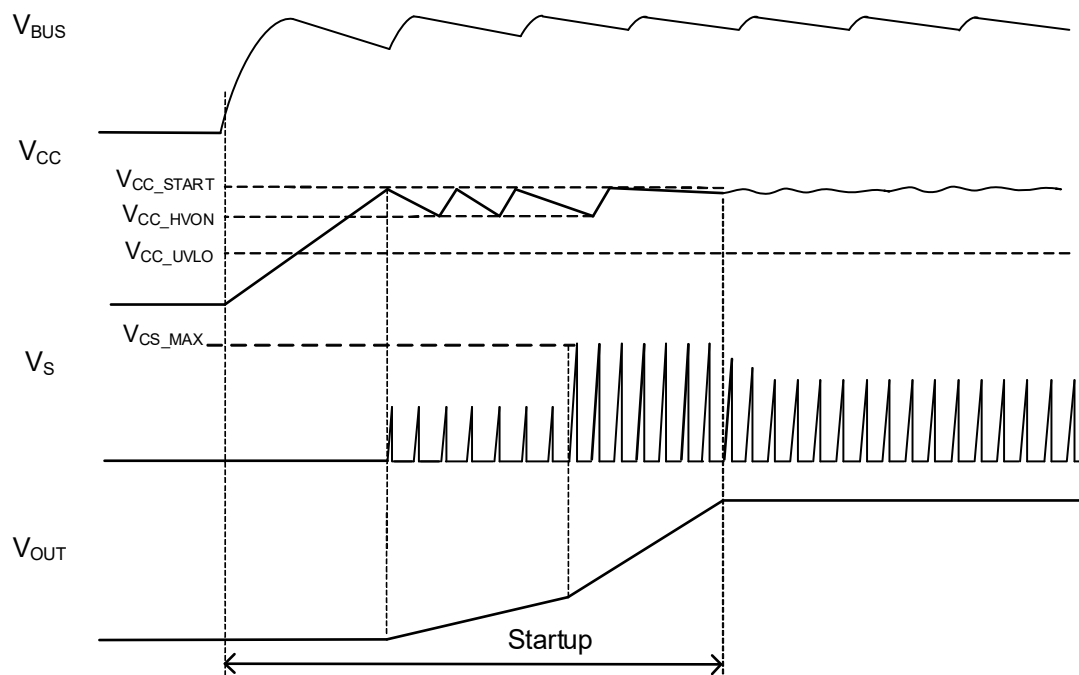
Figure 24. Start-Up Diagram
