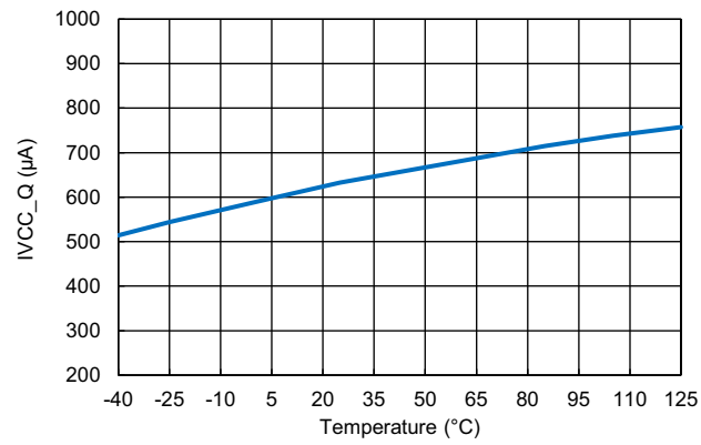
Figure 8. V CC Quiescent Current vs Temperature
