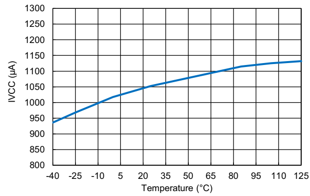
Figure 9. V CC Supply Current in Switching vs Temperature
