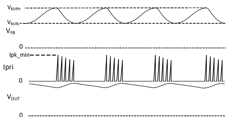
Figure 23. Burst Mode Operation at Light Load
