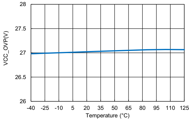
Figure 11. V CC Overvoltage Protection Threshold vs Temperature
