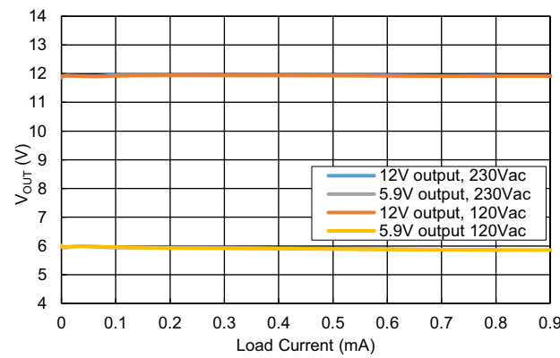
Figure 13. Load Regulation
