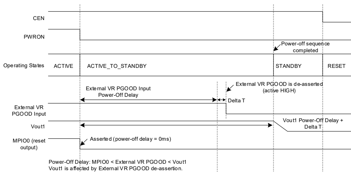
Figure 18. Power-Off Example - External VR PGOOD Input
