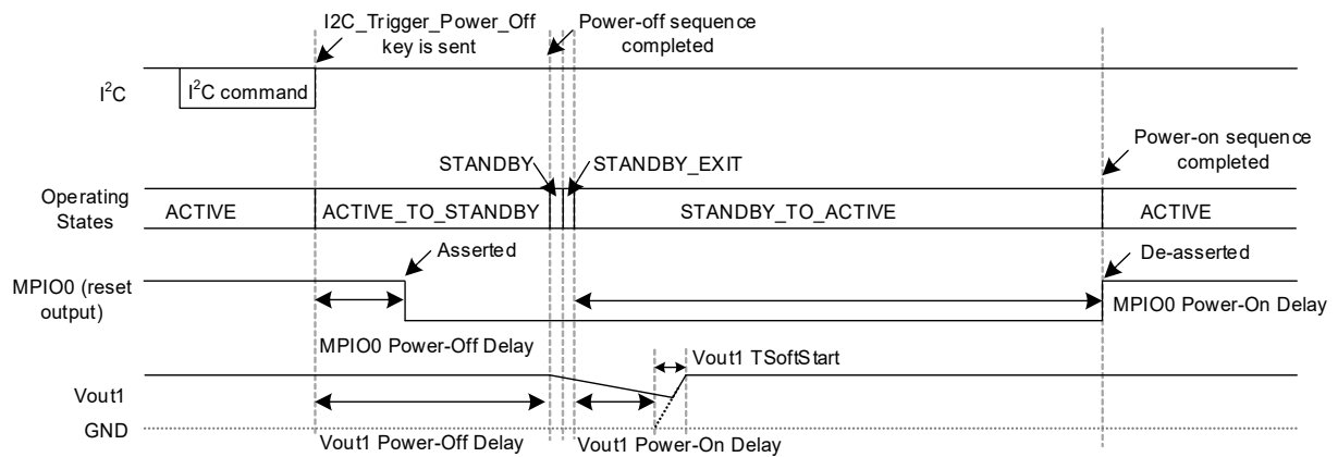
Figure 27. I2C Triggered Power-Off - PWRON = HIGH. PWRON as On/Off Switch, Active HIGH
