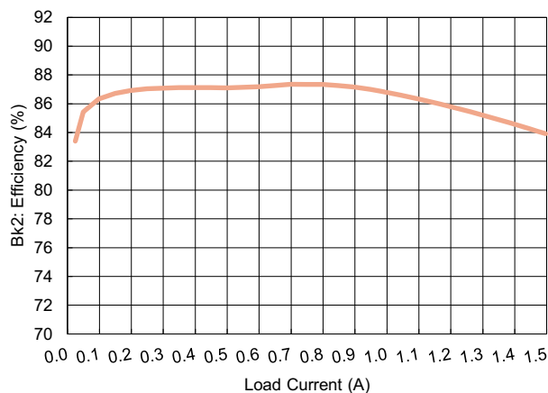
Figure 6. Buck2 Efficiency in Auto PFM/PWM mode
