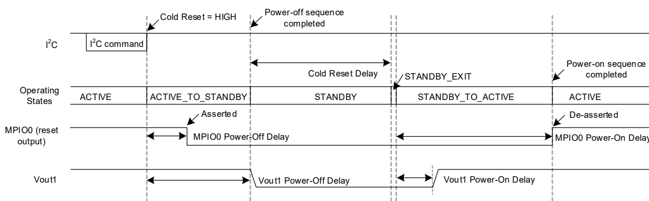
Figure 30. Cold Reset Operation
