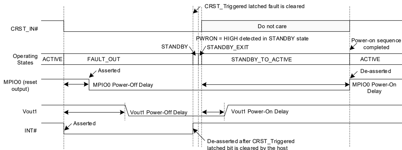
Figure 20. Example of CRST_IN# Operation - CRST_FAULT_EN = Enabled
