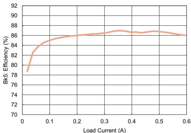
Figure 9. Buck5 Efficiency in Auto PFM/PWM mode
