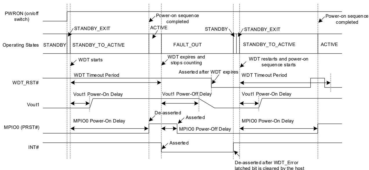
Figure 22. Example of WDT RST# Operation - WD PD EN bit = Enabled
