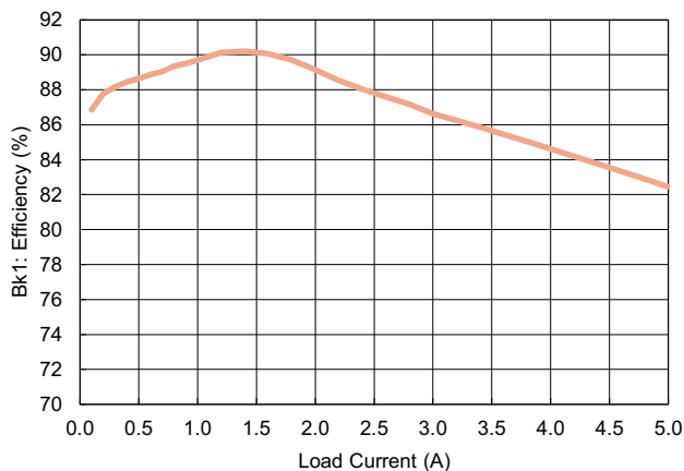
Figure 5. Buck1 Efficiency in Auto PFM/PWM mode
