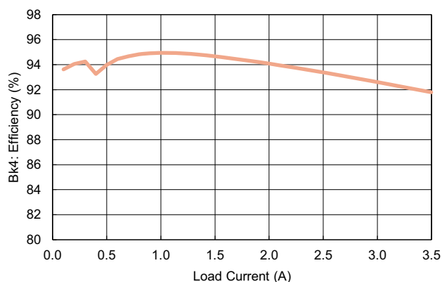
Figure 8. Buck4 Efficiency in Auto PFM/PWM mode
