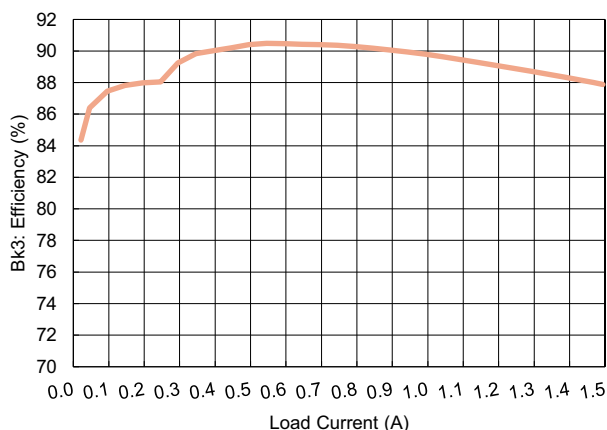
Figure 7. Buck3 Efficiency in Auto PFM/PWM mode
