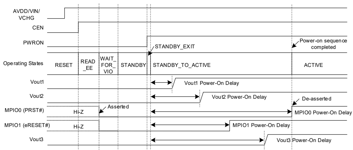
Figure 23. Typical Power-On Example - PWRON as On/Off Switch
