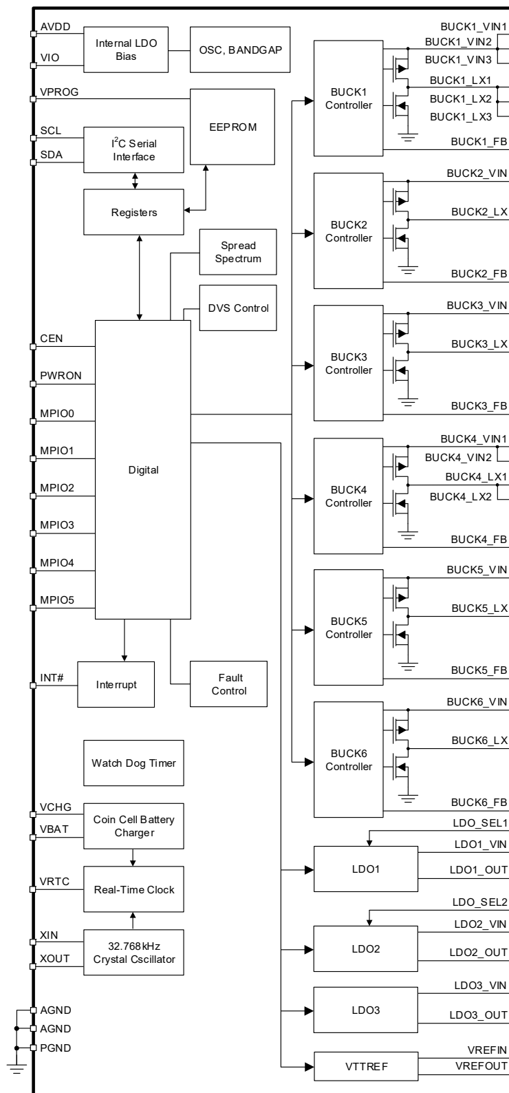
Figure 4. Block Diagram
