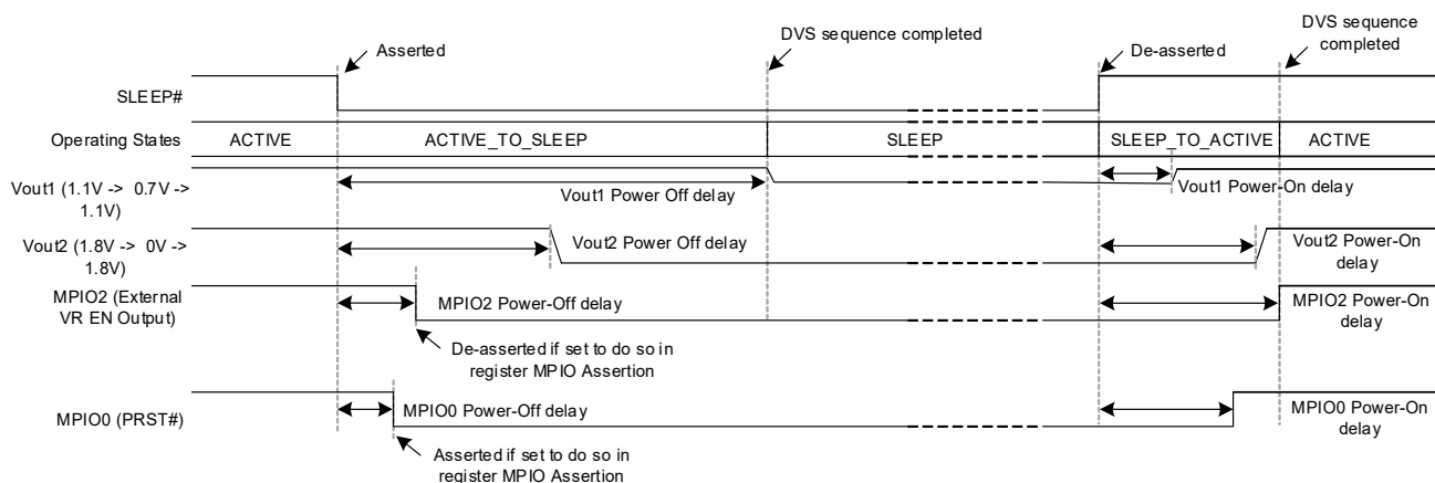
Figure 31. {ACTIVE} <-> {SLEEP} DVS Transition Example
