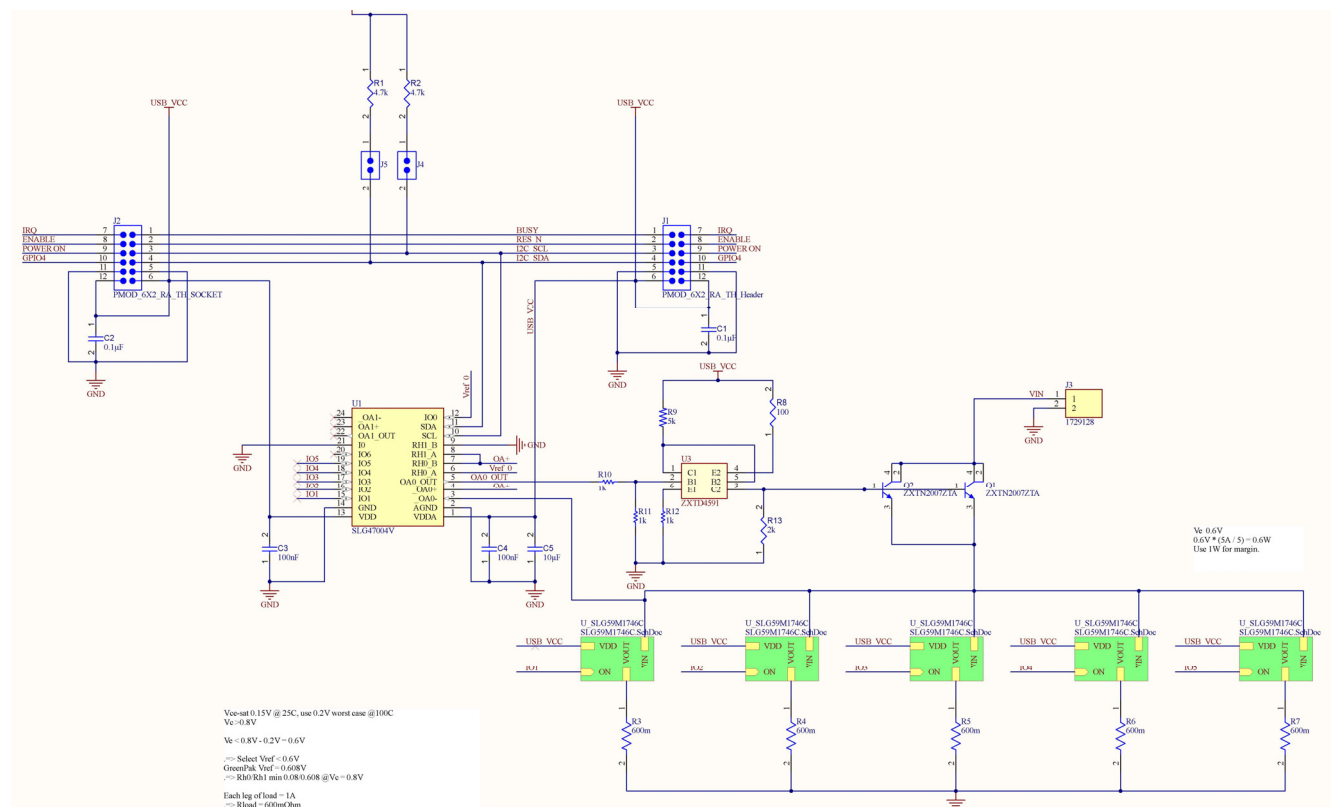
Figure 7. QCIOT-ELOADPOCZ Schematic
