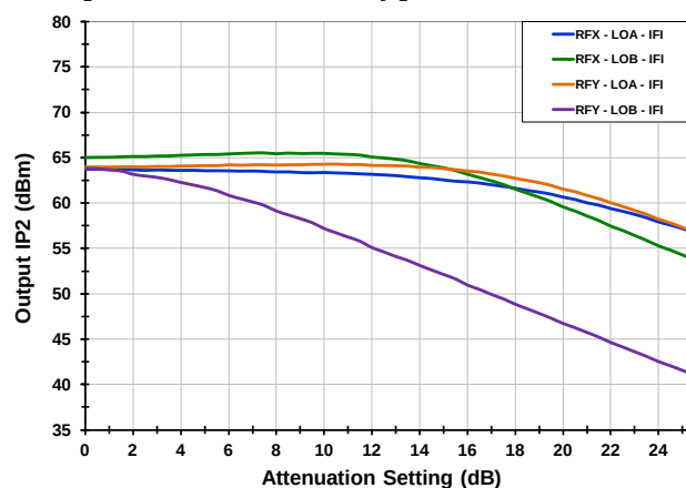
IP2 o [1.0 GHz RF, HiSide Inj.]
