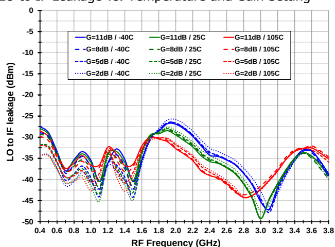
LO to IF Leakage vs. Temperature and Gain Setting
