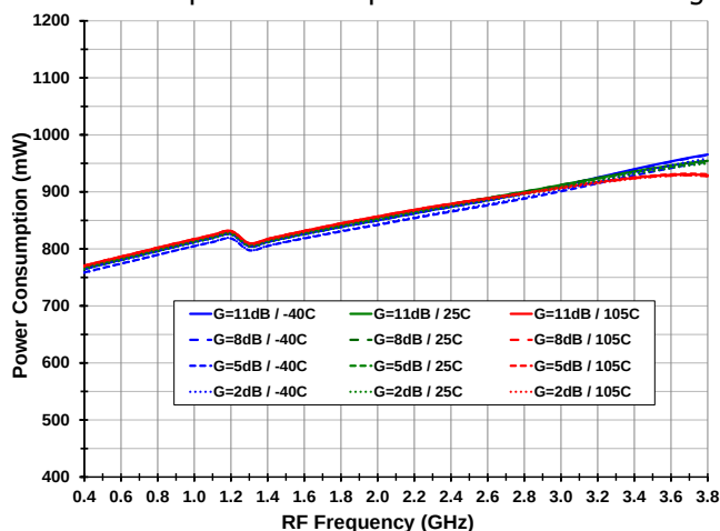
Power Consumption vs. Temperature and Gain Setting
