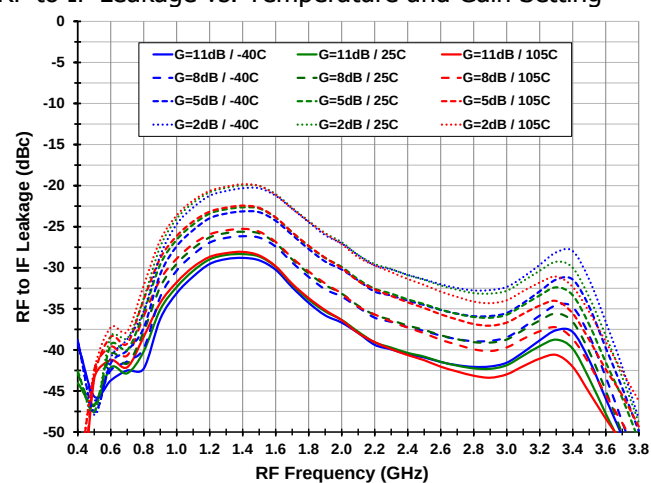
RF to IF Leakage vs. Temperature and Gain Setting
