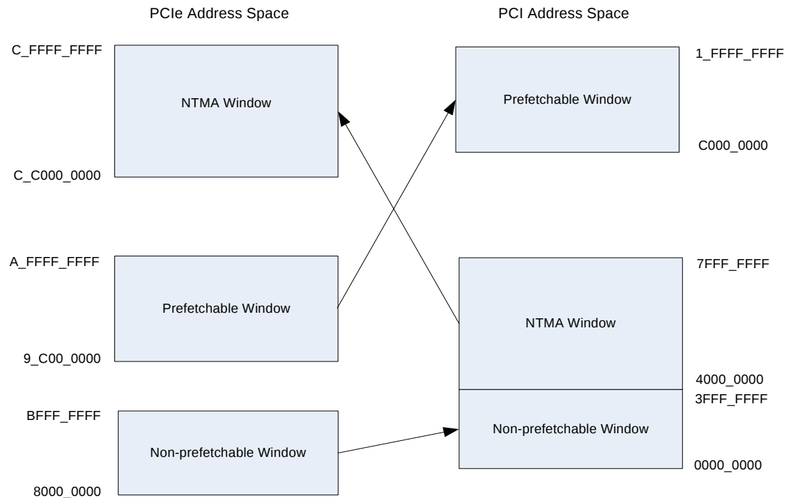
Figure 13: Memory Window Remapping Example
