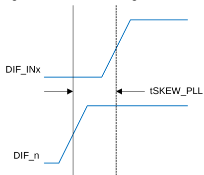
Figure 1. Skew Diagram
