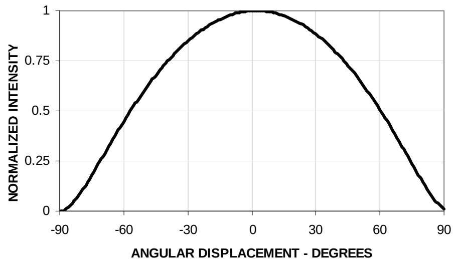
Radiation Diagram
