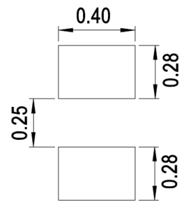
Figure 7: Recommended Soldering Land Pattern
