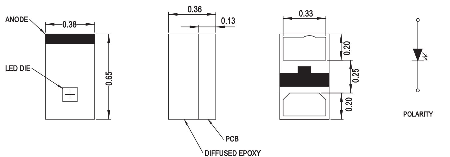
Figure 1: Package Drawing
