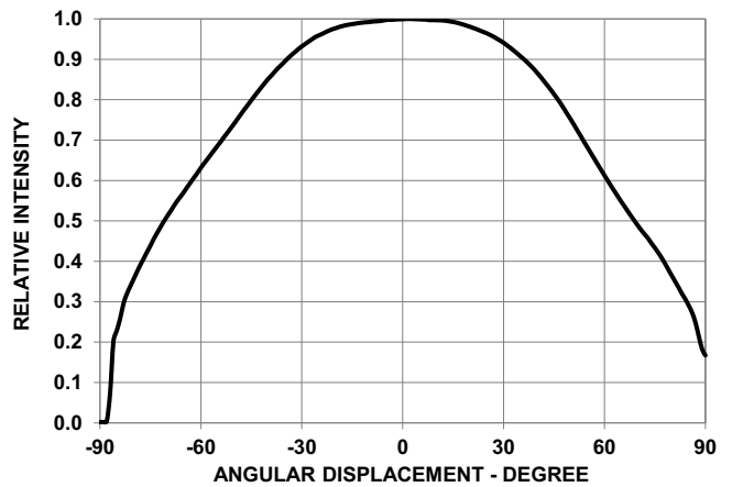
Figure 5: Radiation Pattern
