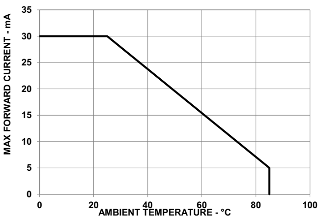
Figure 6: Derating Curve
