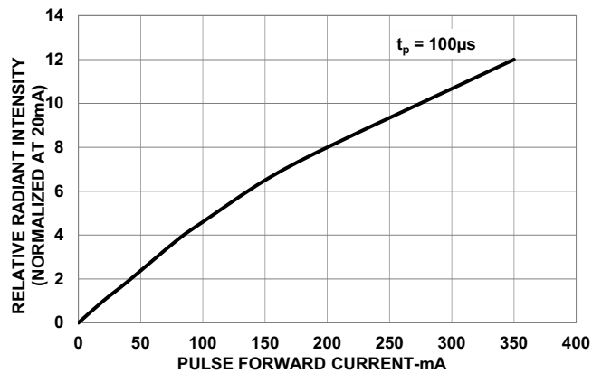
Figure 4: Relative Radiant Intensity vs. Forward Current
