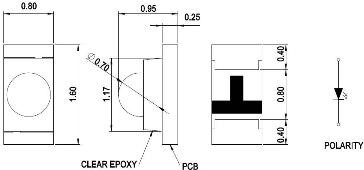
Figure 1: Package Dimensions
