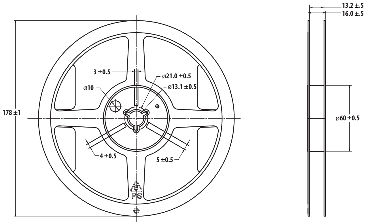
Figure 19: Reel Dimensions
