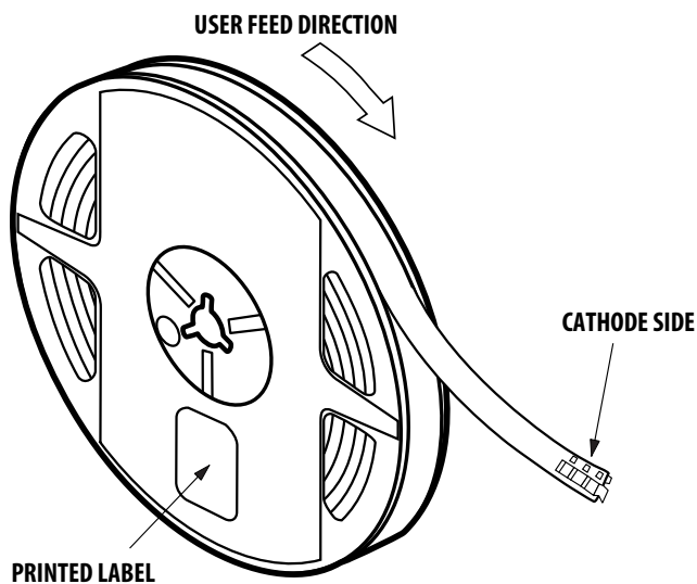
Figure 20: Reeling Orientation
