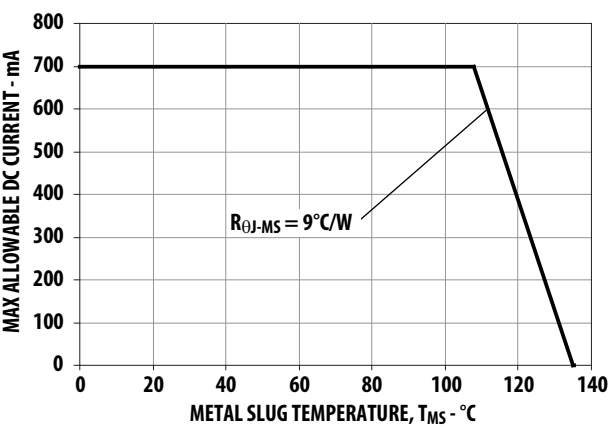
Figure 14: Maximum Forward Current vs. Metal Slug Temperature. Derated Based on T_{JMAX} = 125^{\circ}C , R_{\theta J-MS} = 9^{\circ}C/W .
