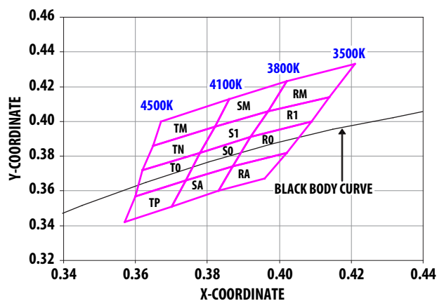
Figure 3: Color Bin Structure for Neutral White
