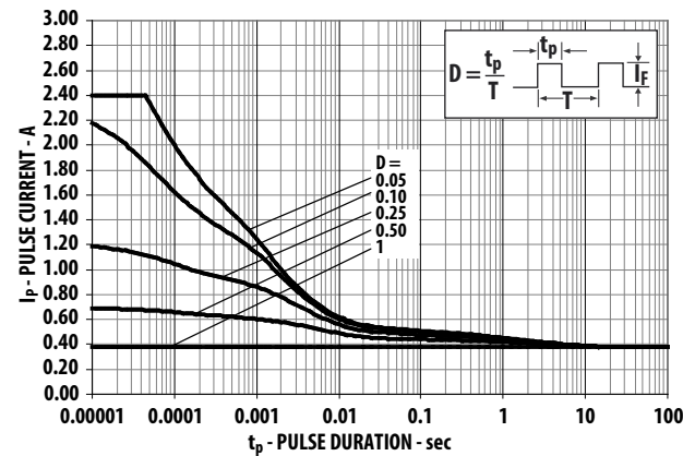
Figure 9: Maximum Pulse Current vs. Pulse Duration. Derated Based on T_A = 85^{\circ}\text{C} , R_{\theta\text{J-A}} = 30^{\circ}\text{C/W} .
