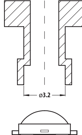
Figure 16: Recommended Pick-and-Place Nozzle Tip. Inner Diameter = 3.2 mm.
