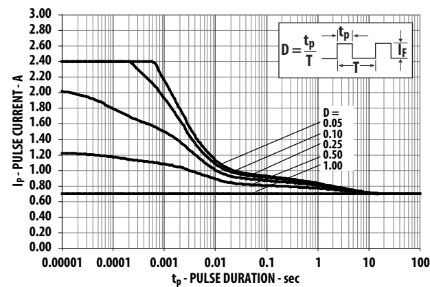
Figure 8: Maximum Pulse Current vs. Pulse Duration. Derated Based on T_A = 25^{\circ}\text{C} , R_{\theta\text{J-A}} = 30^{\circ}\text{C/W} .
