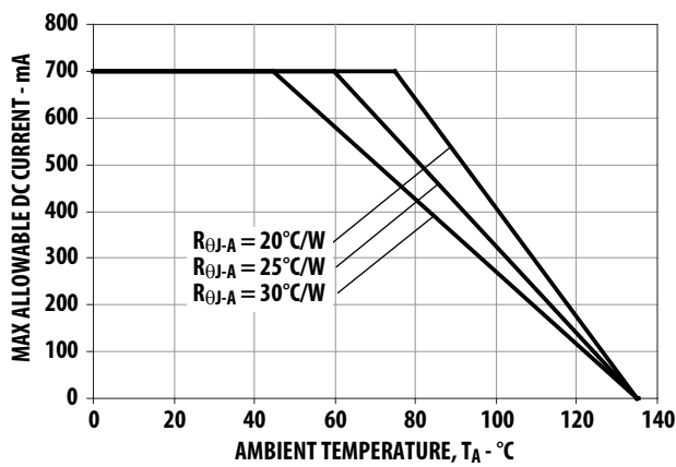
Figure 13: Maximum Forward Current vs. Ambient Temperature. Derated Based on T_{JMAX} = 125^{\circ}C , R_{\theta J-A} = 20^{\circ}C/W , 25^{\circ}C/W , and 30^{\circ}C/W .
