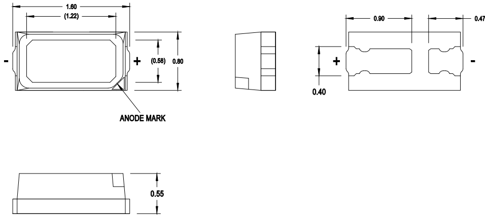
Figure 1: Package Drawing
