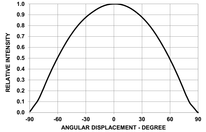
Figure 6: Radiation Pattern
