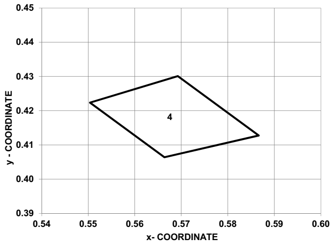
Figure 2: Chromaticity Diagram
