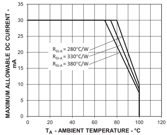
Figure 16: Maximum Forward Current vs. Ambient Temperature. Derated Based on T_{JMAX} = 110^{\circ}C (PC Amber)
