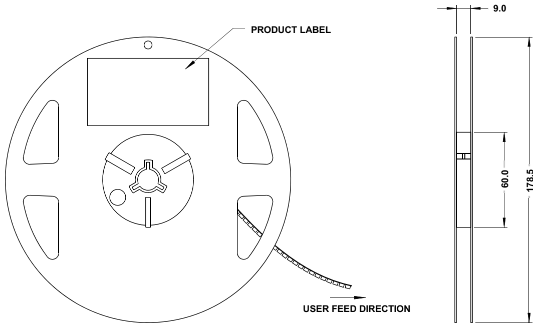
Figure 20: Reel Dimensions
