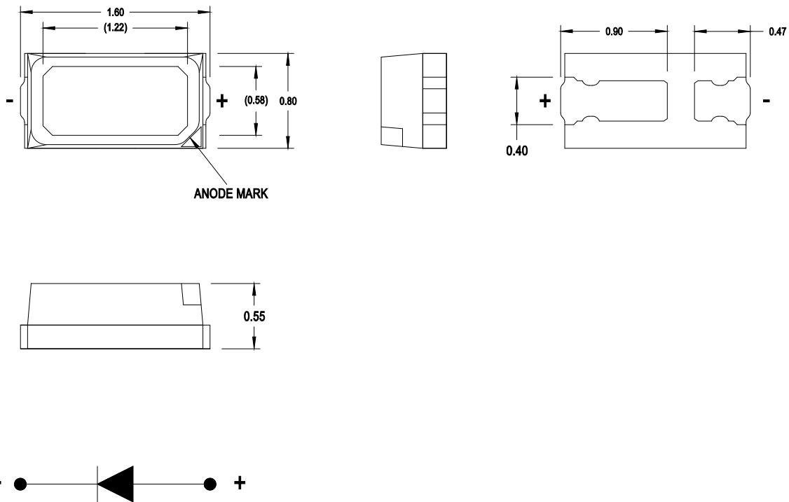
Figure 1: Package Drawing
