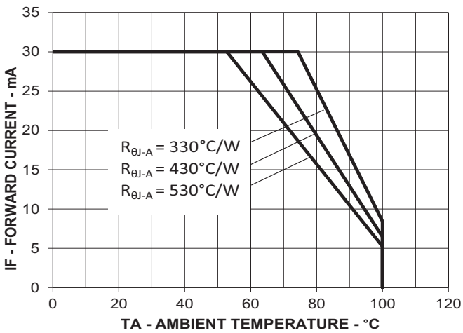
Figure 11: Maximum Forward Current vs. Ambient Temperature. Derated Based on T_{JMAX} = 110^\circ\text{C}
