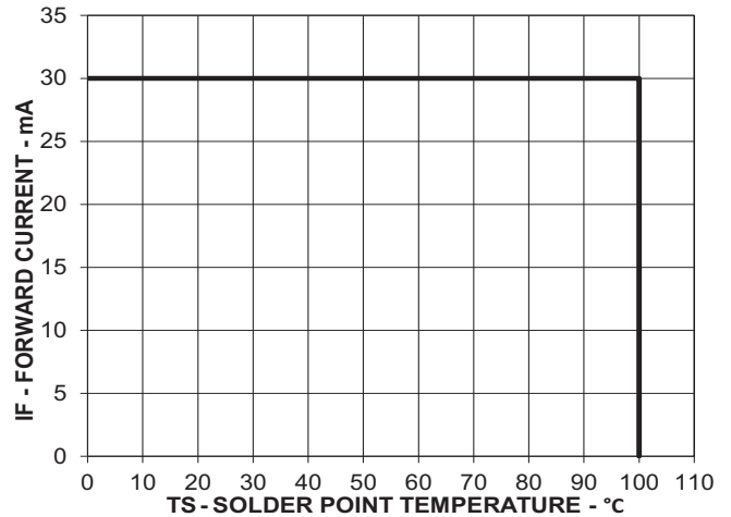
Figure 12: Maximum Forward Current vs. Solder Point Temperature. Derated Based on T_{JMAX} = 110^\circ\text{C}
