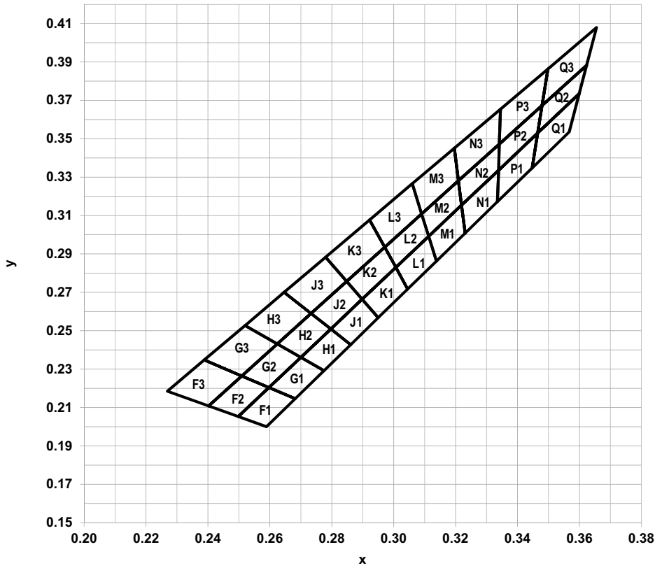
Figure 2: Chromaticity Diagram
