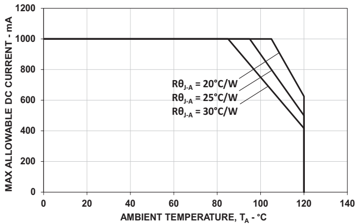
Figure 8: Maximum Forward Current vs. Ambient Temperature for ARE6-8xC1
