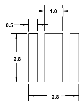
Figure 14: Recommended Soldering Land Pattern
