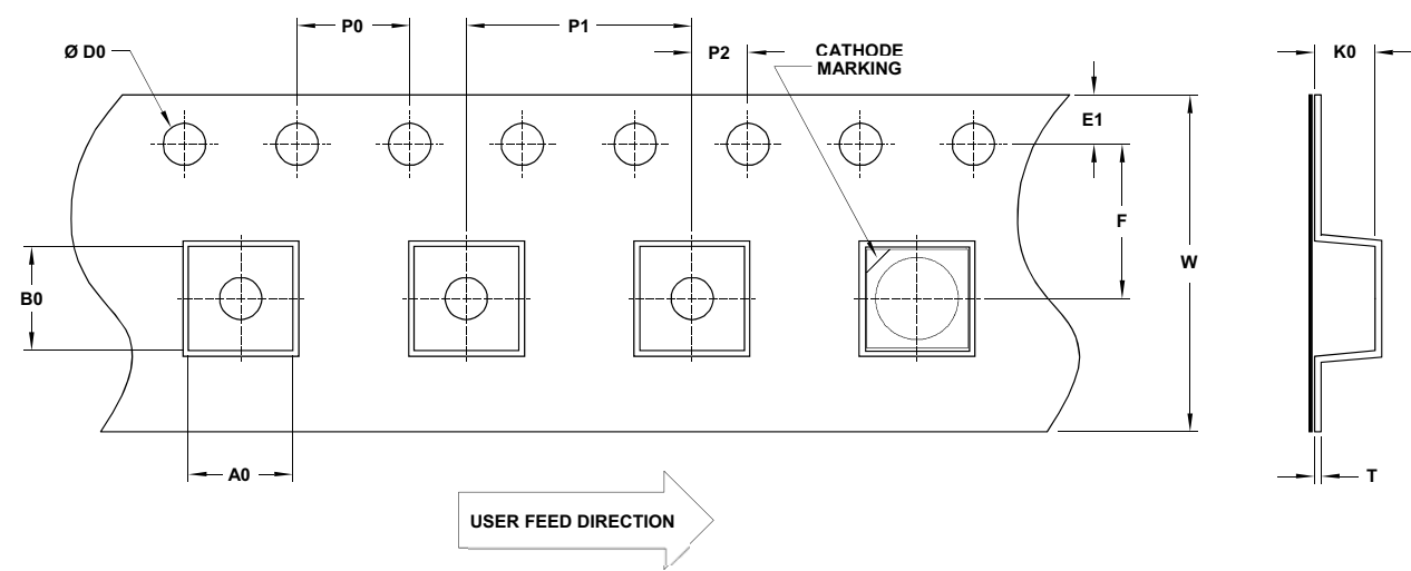
Figure 16: Carrier Tape Dimensions for Viewing Angle 140°
