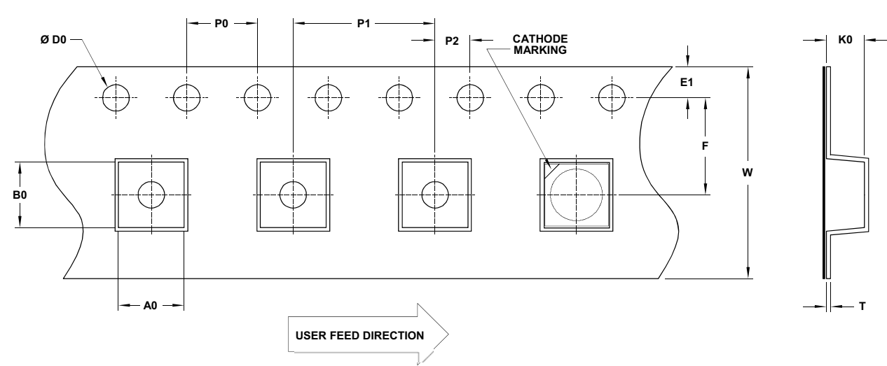
Figure 15: Carrier Tape Dimensions for Viewing Angle 80°
