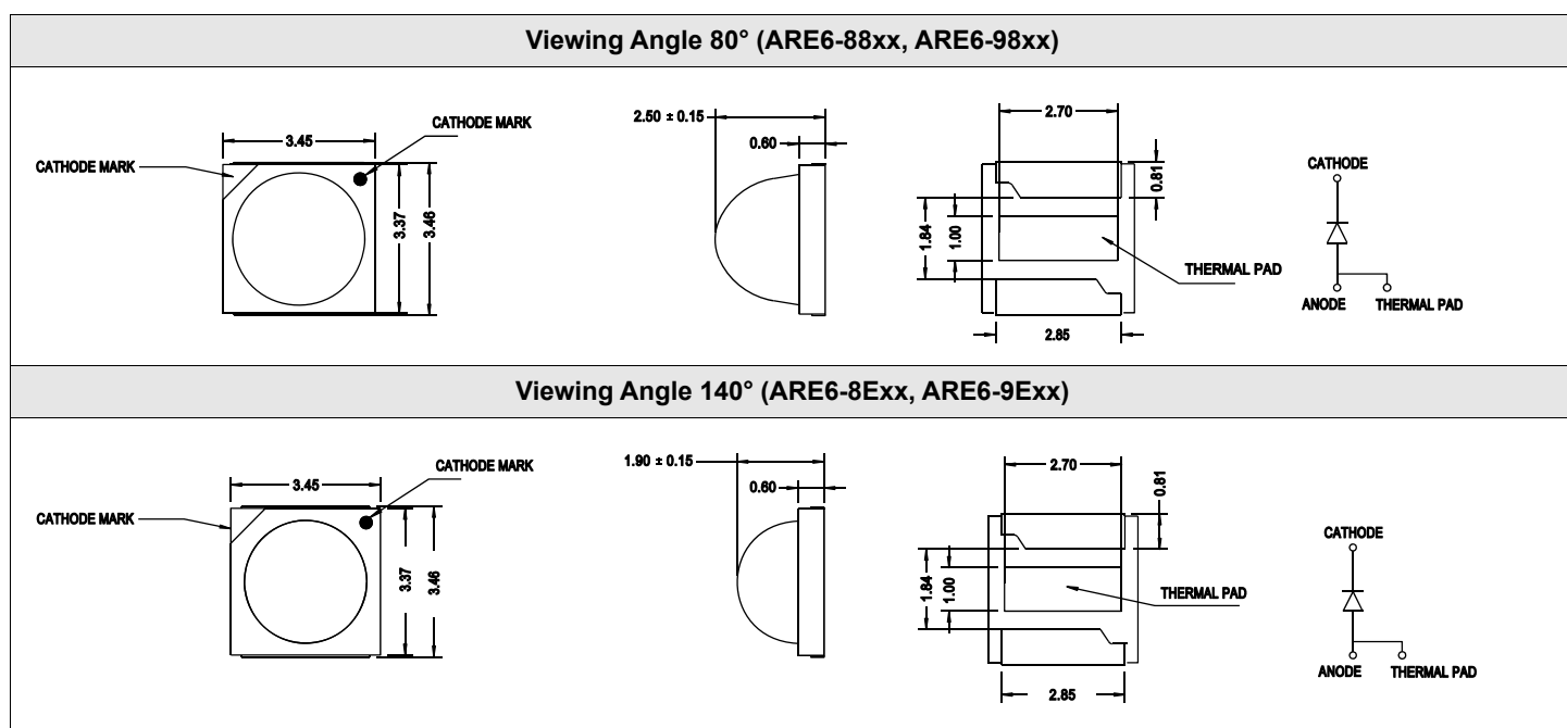
Figure 1: Package Drawing
