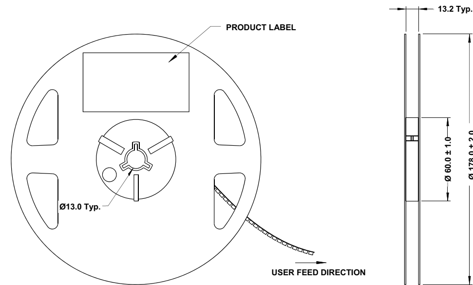
Figure 17: Reel Dimensions
