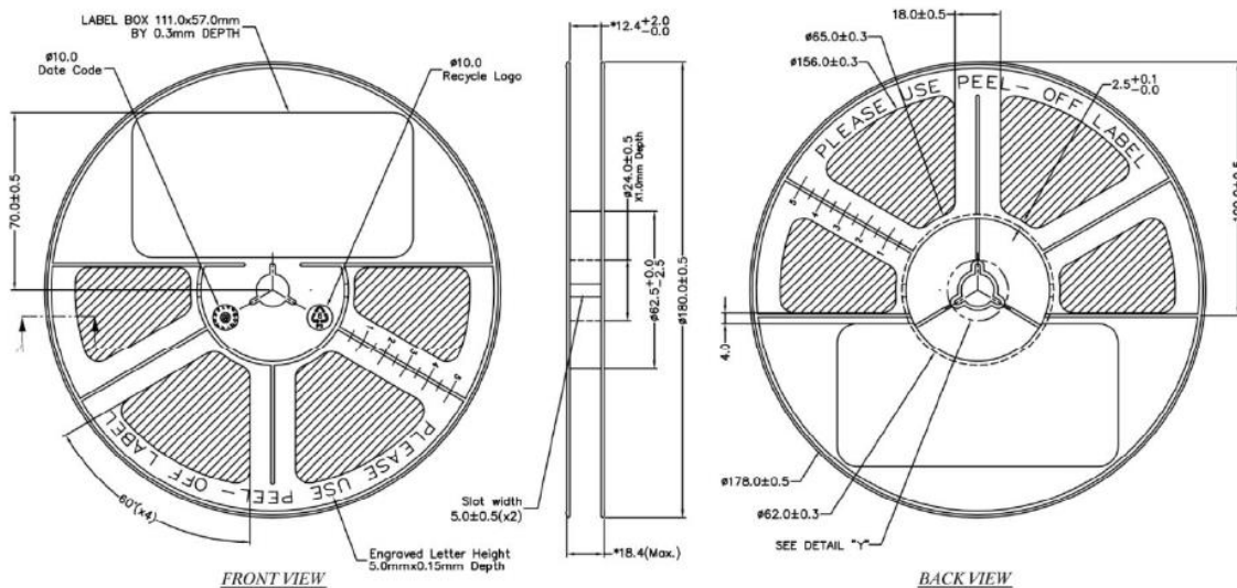
Figure 7: Reel Dimensions
