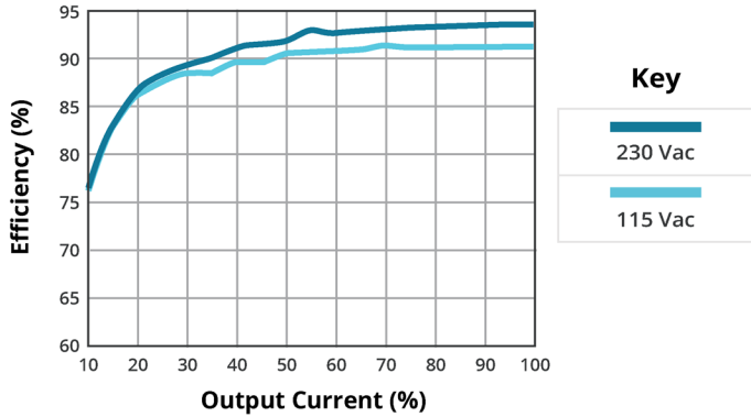
EFFICIENCY VS OUTPUT LOAD TJ-150-48
