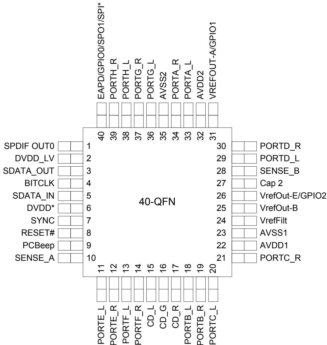
Figure 17. Pin Assignment
