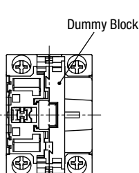
2/4 contact blocks
