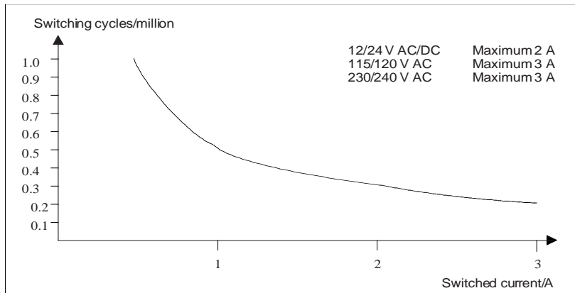
Figure A Switching capacity and service life of the contacts at ohmic load (heating)
