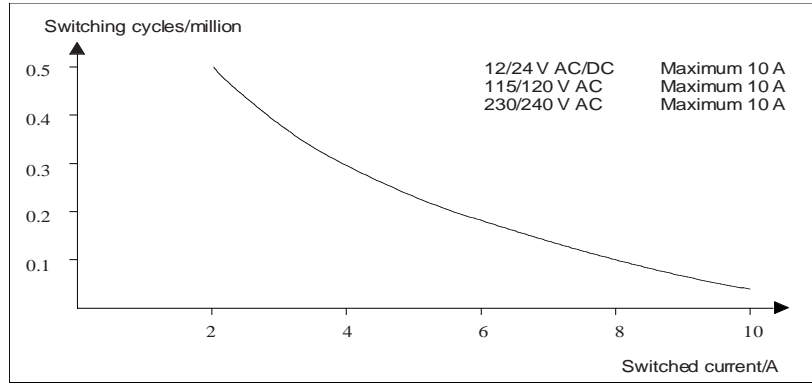
Figure B Switching capacity and service life of the contacts at highly inductive load to IEC 947-5-1 DC13/AC15 (contactors, solenoid coils, motors)
