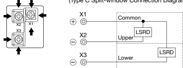
(Type C Split-window Connection Diagram)
