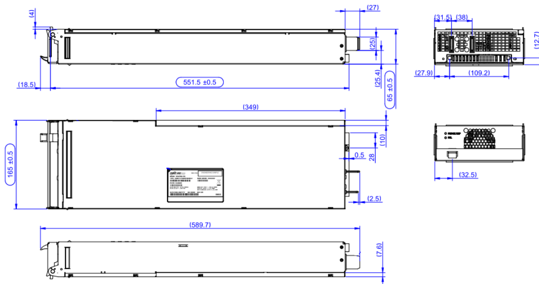
Figure 24. Mechanical Drawing
