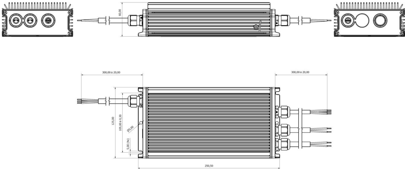
Figure 3. Mechanical drawing
