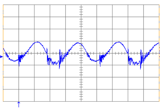
Figure 10. Output voltage ripple (20mV/div.) at full rated load current into a resistive load with C_o = 10\mu\text{F tantalum} + 1\mu\text{F ceramic} and V_{in} = 48\text{ V} . Time scale: 1µs/div.
