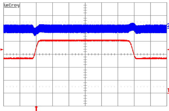
Figure 8. Output voltage response to load current step-change (12.5A–18.75A–12.5A) at V_{in} = 48\text{ V} . Top trace: output voltage (100mV/div.). Bottom trace: load current (5A/div.). Current slew rate: 0.1A/µs. C_o = 1\mu\text{F cer} + 10\mu\text{F tant} . Time scale: 0.2ms/div.
