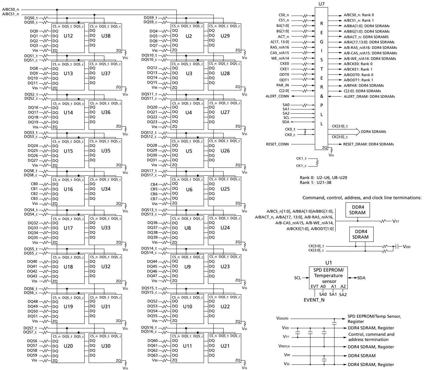
Figure 4: Functional Block Diagram, R/C-B2 (PCBs 1971, 2436, or 2615)
