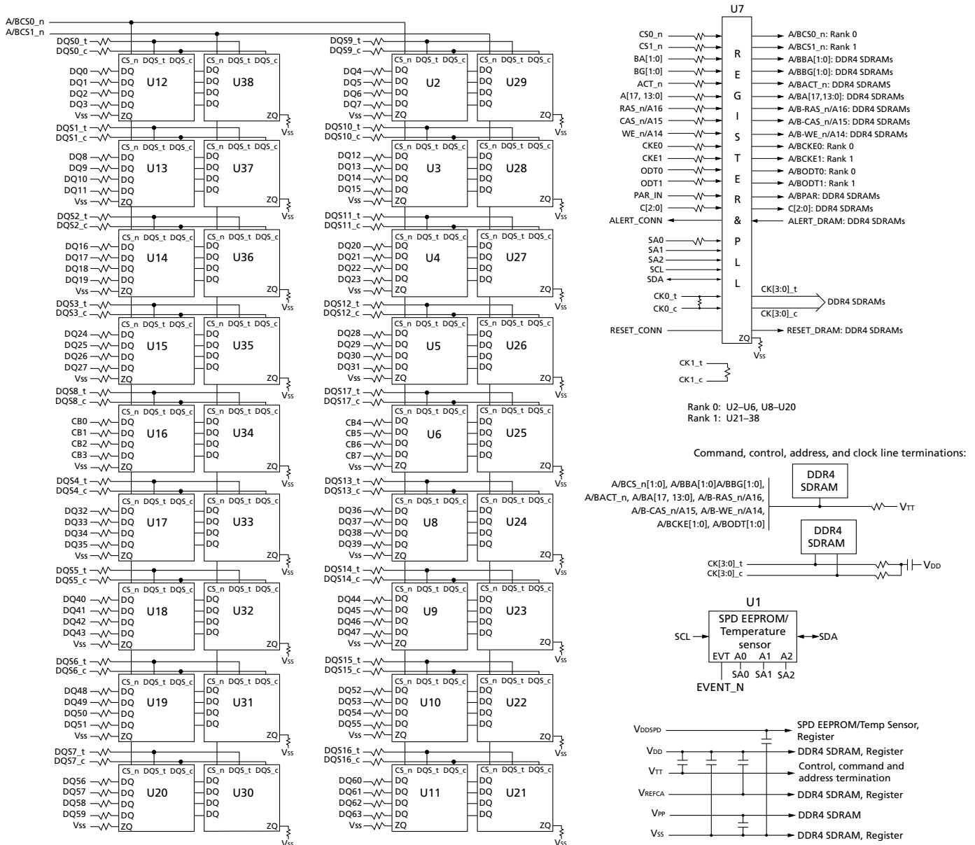
Figure 4: Functional Block Diagram, R/C-B2 (PCB 1971)
