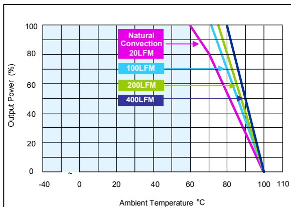
Figure 27: AXA00B18-L Derating Curves (without heatsink) Vin = 24Vdc Load: Io = 0 to 0.83A
