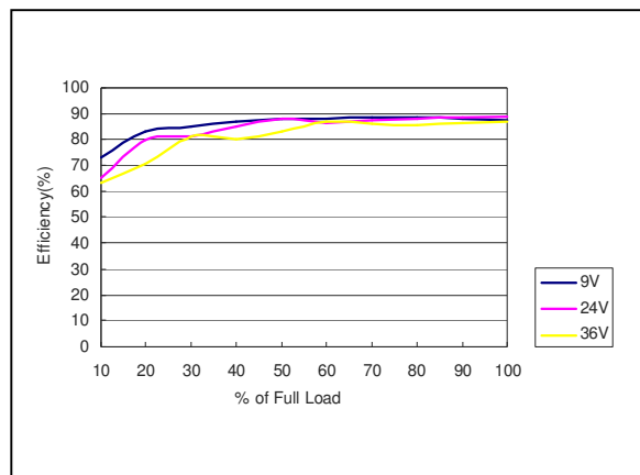
Figure 71: AXA000CC18-L Efficiency Versus Output Current Curve Vin = 9 to 36Vdc Load: Io = 0 to \pm 0.33 A
