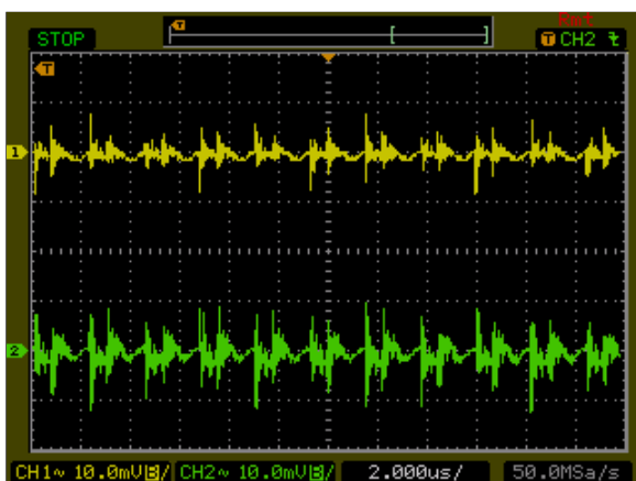
Figure 143: AXA000BB36-L Ripple and Noise Measurement Vin = 48Vdc Load: Io = \pm 0.41 A Ch 1: Vo
