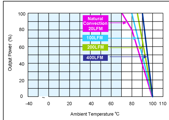
Figure 138: AXA00AA36-L Derating Curves (with heatsink) Vin = 48Vdc Load: Io = 0 to ±1 A
