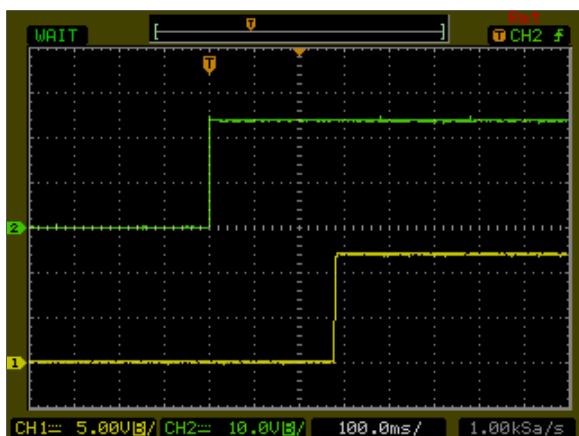
Figure 25: AXA00B18-L Output Voltage Startup Characteristic by ON/OFF Vin = 24Vdc Load: Io = 0.83A Ch1: Vo Ch2: Remote On/Off
