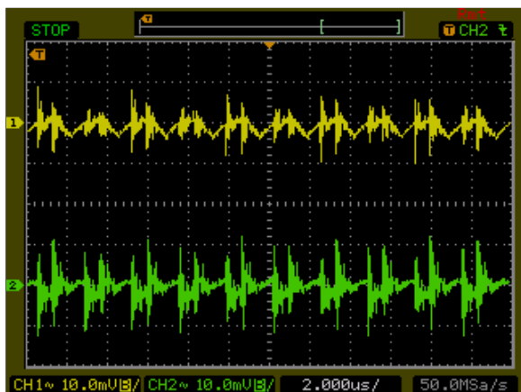
Figure 153: AXA000CC36-L Ripple and Noise Measurement Vin = 48Vdc Load: Io = \pm 0.33 A Ch 1: Vo
