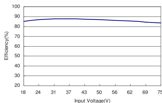
Figure 82: AXA02F36-L Efficiency Versus Input Voltage Curve Vin = 18 to 75Vdc Load: Io = 2.2A
