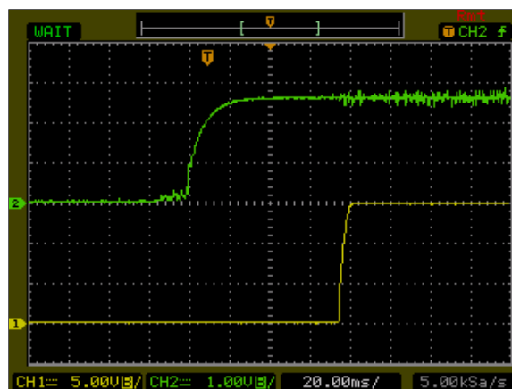
Figure 156: AXA000CC36-L Output Voltage Startup Characteristic by Vin Vin = 48Vdc Load: Io = \pm 0.33 A Ch1: Vo Ch2: Vin
