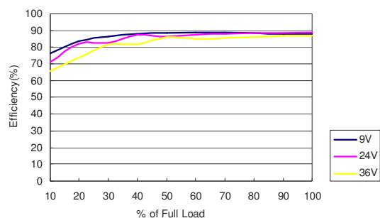
Figure 21: AXA00B18-L Efficiency Versus Output Current Curve Vin = 9 to 36Vdc Load: Io = 0 to 0.83A
