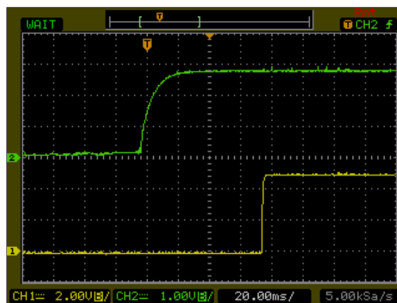
Figure 16: AXA02A18-L Output Voltage Startup Characteristic by Vin Vin = 24Vdc Load: Io = 2A Ch1: Vo Ch2: Vin
