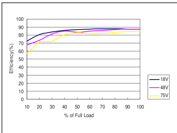
Figure 141: AXA000BB36-L Efficiency Versus Output Current Curve Vin = 18 to 75Vdc Load: Io = 0 to \pm 0.41 A
