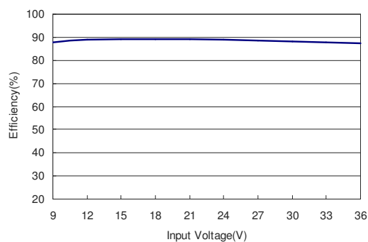
Figure 22: AXA00B18-L Efficiency Versus Input Voltage Curve Vin = 9 to 36Vdc Load: Io = 0.83A
