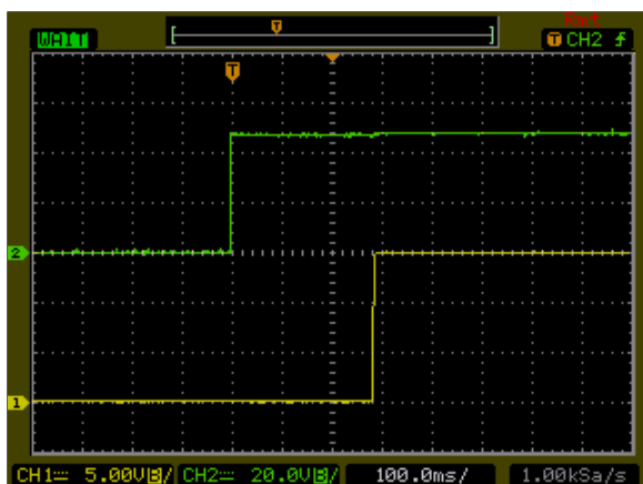
Figure 155: AXA000CC36-L Output Voltage Startup Characteristic by ON/OFF Vin = 48Vdc Load: Io = \pm 0.33 A Ch1: Vo Ch2: Remote On/Off
