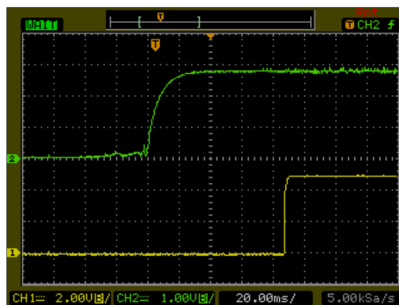
Figure 96: AXA02A36-L Output Voltage Startup Characteristic by Vin Vin = 48Vdc Load: Io = 2A Ch1: Vo Ch2: Vin
