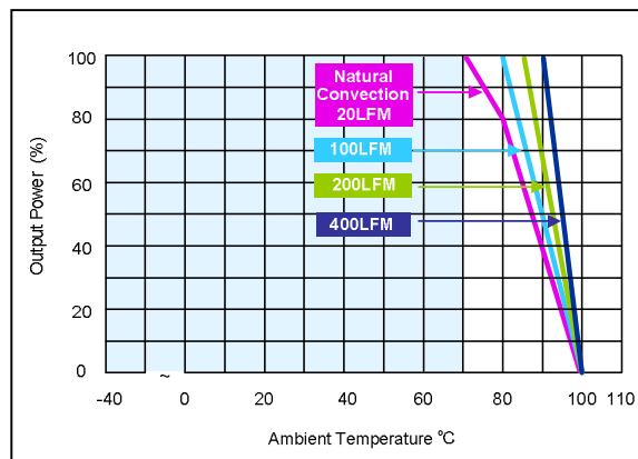
Figure 18: AXA02A18-L Derating Curves (with heatsink) Vin = 24Vdc Load: Io = 0 to 2A
