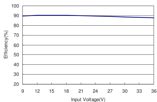
Figure 32: AXA00C18-L Efficiency Versus Input Voltage Curve Vin = 9 to 36Vdc Load: Io = 0.67A
