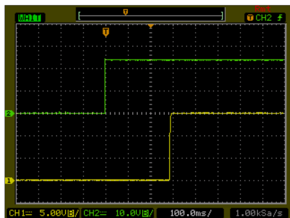
Figure 75: AXA000CC18-L Output Voltage Startup Characteristic by ON/OFF Vin = 24Vdc Load: Io = \pm 0.33 A Ch1: Vo Ch2: Remote On/Off
