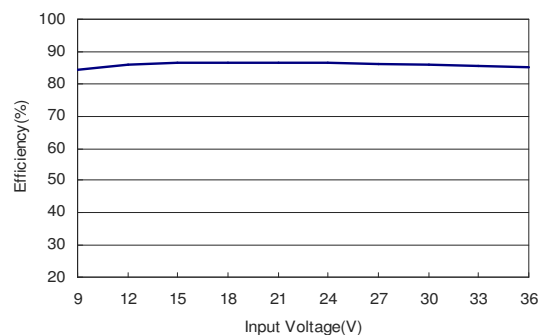
Figure 52: AXA00AA18-L Efficiency Versus Input Voltage Curve Vin = 9 to 36Vdc Load: Io = \pm 1 A
