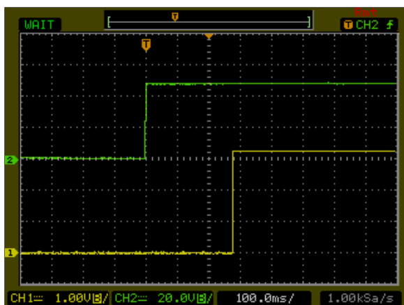
Figure 85: AXA02F36-L Output Voltage Startup Characteristic by ON/OFF Vin = 48Vdc Load: Io = 2.2A Ch1: Vo Ch2: Remote On/Off
