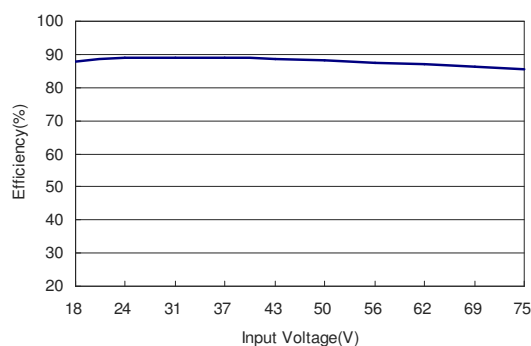
Figure 112: AXA00C36-L Efficiency Versus Input Voltage Curve Vin = 18 to 75Vdc Load: Io = 0.67A
