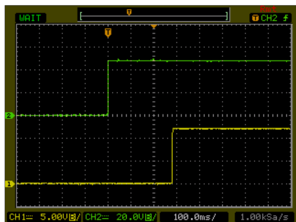
Figure 105: AXA00B36-L Output Voltage Startup Characteristic by ON/OFF Vin = 48Vdc Load: Io = 0.83A Ch1: Vo Ch2: Remote On/Off
