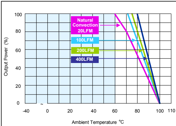
Figure 87: AXA02F36-L Derating Curves (without heatsink) Vin = 48Vdc Load: Io = 0 to 2.2A
