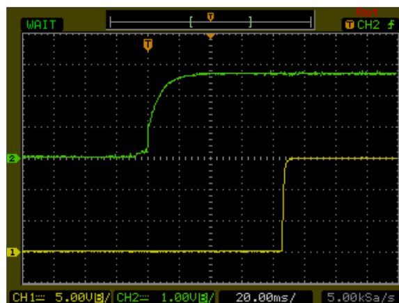
Figure 36: AXA01C18-L Output Voltage Startup Characteristic by Vin Vin = 24Vdc Load: Io = 1.33A Ch1: Vo Ch2: Vin
