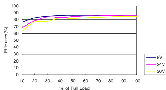
Figure 51: AXA00AA18-L Efficiency Versus Output Current Curve Vin = 9 to 36Vdc Load: Io = 0 to \pm 1 A
