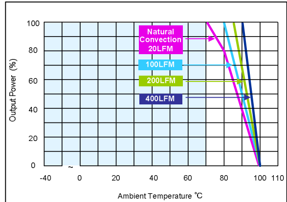
Figure 98: AXA02A36-L Derating Curves (with heatsink) Vin = 48Vdc Load: Io = 0 to 2A
