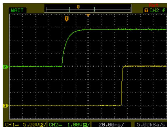
Figure 116: AXA00C36-L Output Voltage Startup Characteristic by Vin Vin = 48Vdc Load: Io = 0.67A Ch1: Vo Ch2: Vin
