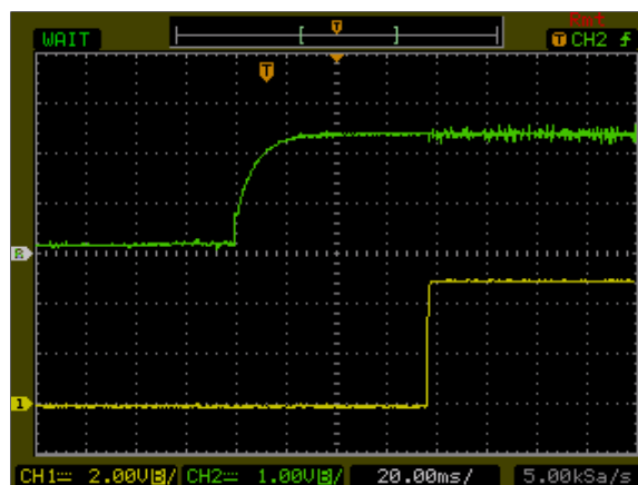
Figure 136: AXA00AA36-L Output Voltage Startup Characteristic by Vin Vin = 48Vdc Load: Io = ±1 A Ch1: Vo Ch2: Vin
