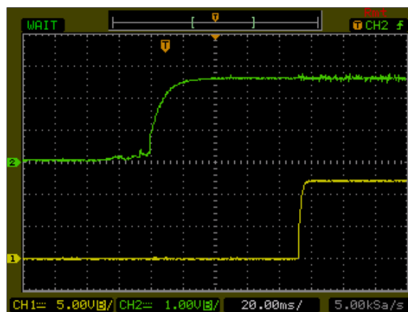
Figure 65: AXA000BB18-L Output Voltage Startup Characteristic by Vin Vin = 24Vdc Load: Io = \pm 0.41 A Ch1: Vo Ch2: Vin
