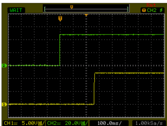
Figure 145: AXA000BB36-L Output Voltage Startup Characteristic by ON/OFF Vin = 48Vdc Load: Io = \pm 0.41 A Ch1: Vo Ch2: Remote On/Off
