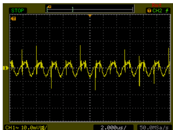
Figure 103: AXA00B36-L Ripple and Noise Measurement Vin = 48Vdc Load: Io = 0.83A Ch 1: Vo
