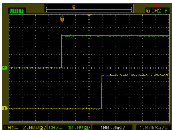
Figure 55: AXA00AA18-L Output Voltage Startup Characteristic by ON/OFF Vin = 24Vdc Load: Io = \pm 1 A Ch1: Vo Ch2: Remote On/Off
