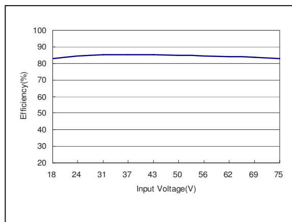
Figure 92: AXA02A36-L Efficiency Versus Input Voltage Curve Vin = 18 to 75Vdc Load: Io = 2A
