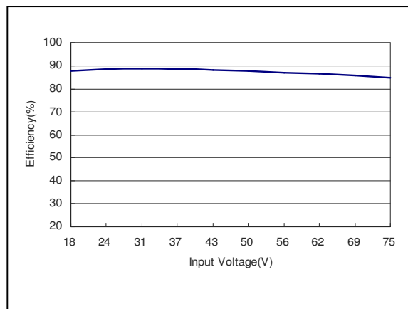
Figure 142: AXA000BB36-L Efficiency Versus Input Voltage Curve Vin = 18 to 75Vdc Load: Io = \pm 0.41 A
