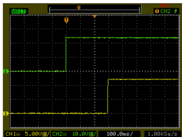
Figure 66: AXA000BB18-L Output Voltage Startup Characteristic by ON/OFF Vin = 24Vdc Load: Io = \pm 0.41 A Ch1: Vo Ch2: Remote On/Off
