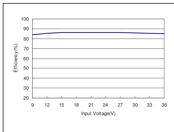
Figure 12: AXA02A18-L Efficiency Versus Input Voltage Curve Vin = 9 to 36Vdc Load: Io = 2A
