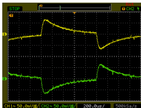
Figure 134: AXA00AA36-L Transient Response Vin = 48Vdc Load: Io = 100% to 75% load change Ch 1: Vo1 Ch2: Vo2
