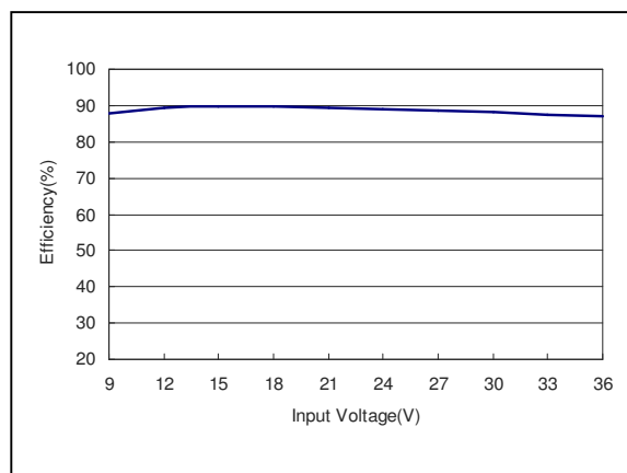
Figure 72: AXA000CC18-L Efficiency Versus Input Voltage Curve Vin = 9 to 36Vdc Load: Io = \pm 0.33 A
