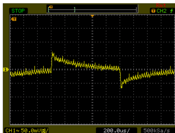
Figure 94: AXA02A36-L Transient Response Vin = 48Vdc Load: Io = 100% to 75% load change Ch 1: Vo
