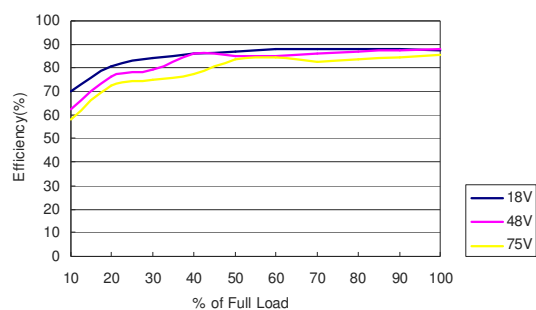
Figure 151: AXA000CC36-L Efficiency Versus Output Current Curve Vin = 18 to 75Vdc Load: Io = 0 to \pm 0.33 A
