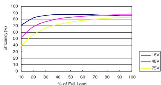
Figure 81: AXA02F36-L Efficiency Versus Output Current Curve Vin = 18 to 75Vdc Load: Io = 0 to 2.2A
