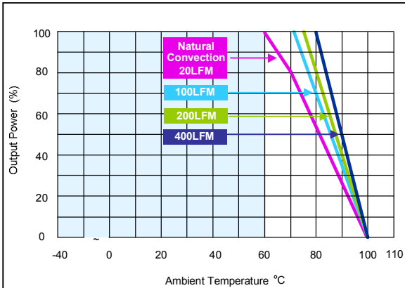
Figure 127: AXA000H36-L Derating Curves (without heatsink) Vin = 48Vdc Load: Io = 0 to 0.41 A
