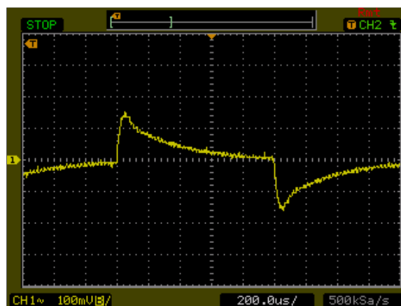
Figure 104: AXA00B36-L Transient Response Vin = 48Vdc Load: Io = 100% to 75% load change Ch 1: Vo
