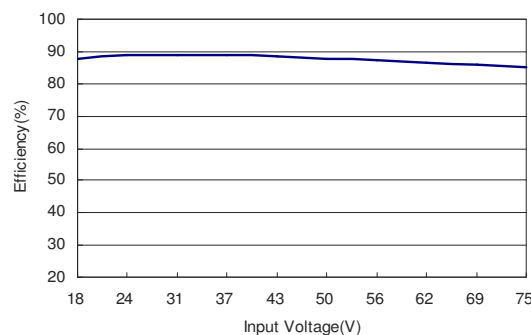
Figure 152: AXA000CC36-L Efficiency Versus Input Voltage Curve Vin = 18 to 75Vdc Load: Io = \pm 0.33 A
