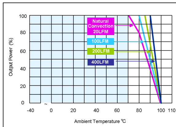
Figure 28: AXA00B18-L Derating Curves (with heatsink) Vin = 24Vdc Load: Io = 0 to 0.83A
