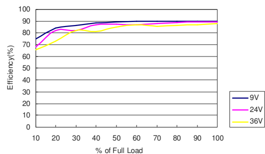
Figure 31: AXA00C18-L Efficiency Versus Output Current Curve Vin = 9 to 36Vdc Load: Io = 0 to 0.67A
