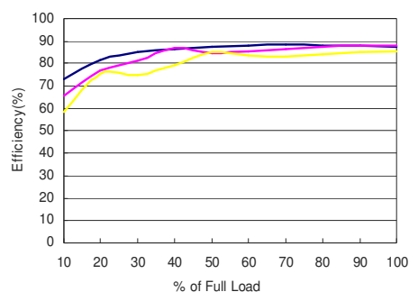
Figure 111: AXA00C36-L Efficiency Versus Output Current Curve Vin = 18 to 75Vdc Load: Io = 0 to 1.33A
