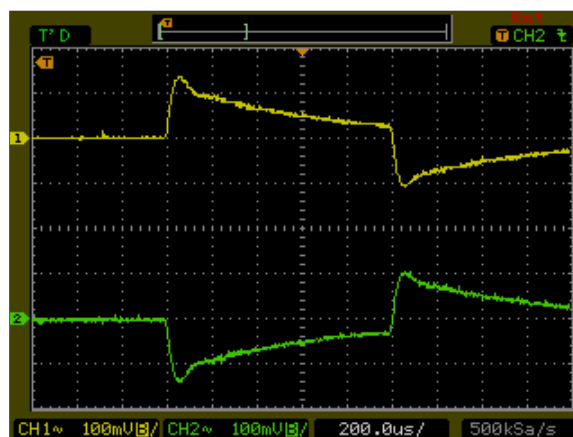
Figure 74: AXA000CC18-L Transient Response Vin = 24Vdc Load: Io = 100% to 75% load change Ch 1: Vo1 Ch2: Vo2
