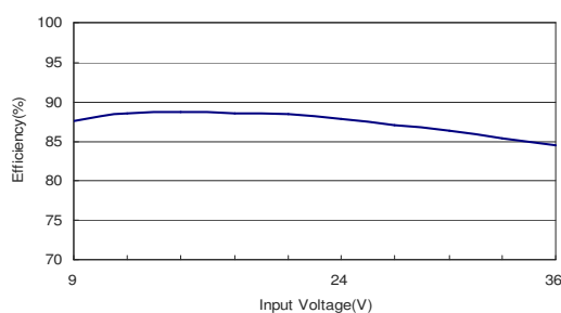
Figure 42: AXA000H18-L Efficiency Versus Input Voltage Curve Vin = 9 to 36Vdc Load: Io = 0.41A
