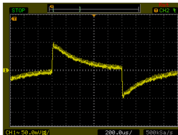
Figure 24: AXA00B18-L Transient Response Vin = 24Vdc Load: Io = 100% to 75% load change Ch 1: Vo
