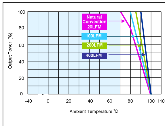
Figure 68: AXA000BB18-L Derating Curves (with heatsink) Vin = 24Vdc Load: Io = 0 to ±0.41 A
