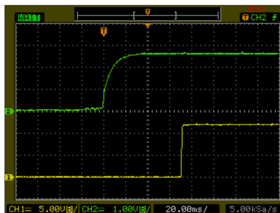
Figure 26: AXA00B18-L Output Voltage Startup Characteristic by Vin Vin = 24Vdc Load: Io = 0.83A Ch1: Vo Ch2: Vin
