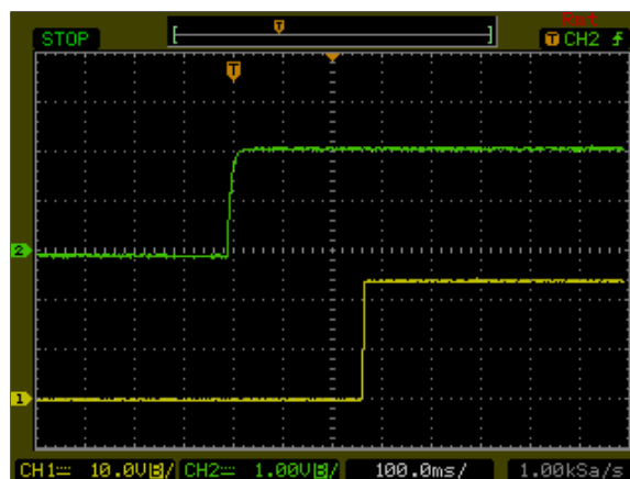
Figure 46: AXA000H18-L Output Voltage Startup Characteristic by Vin Vin = 24Vdc Load: Io = 0.41 Ch1: Vo Ch2: Vin
