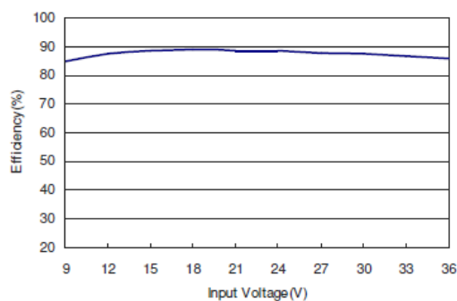
Figure 2: AXA02F18-L Efficiency Versus Input Voltage Curve Vin = 9 to 36Vdc Load: Io = 2.2A
