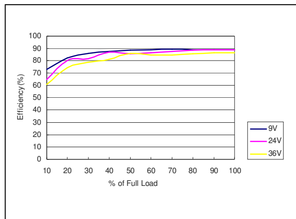
Figure 61: AXA000BB18-L Efficiency Versus Output Current Curve Vin = 9 to 36Vdc Load: Io = 0 to \pm 0.41 A
