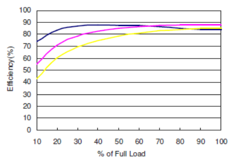
Figure 1: AXA02F18-L Efficiency Versus Output Current Curve Vin = 9 to 36Vdc Load: Io = 0 to 2.2A
