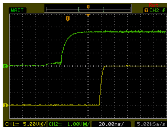
Figure 76: AXA000CC18-L Output Voltage Startup Characteristic by Vin Vin = 24Vdc Load: Io = \pm 0.33 A Ch1: Vo Ch2: Vin
