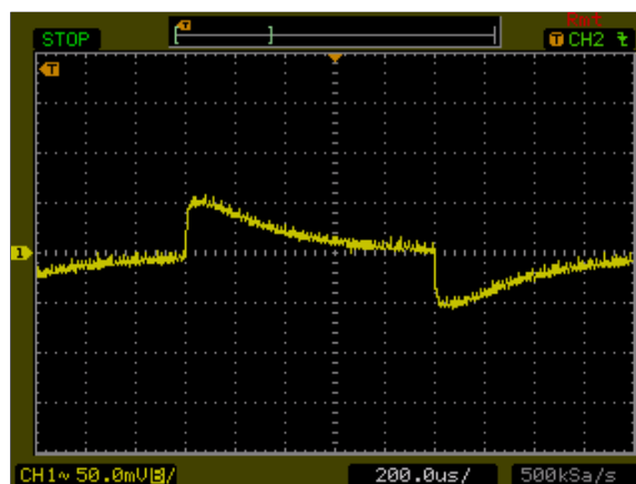
Figure 84: AXA02F36-L Transient Response Vin = 48Vdc Load: Io = 100% to 75% load change Ch 1: Vo
