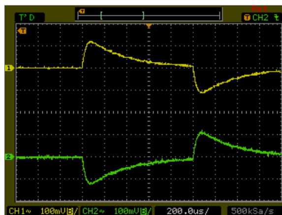
Figure 144: AXA000BB36-L Transient Response Vin = 48Vdc Load: Io = 100% to 75% load change Ch 1: Vo
