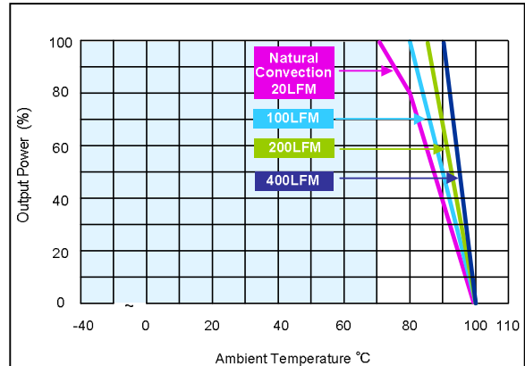
Figure 128: AXA000H36-L Derating Curves (with heatsink) Vin = 48Vdc Load: Io = 0 to 0.41 A
