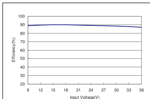
Figure 62: AXA000BB18-L Efficiency Versus Input Voltage Curve Vin = 9 to 36Vdc Load: Io = \pm 0.41 A
