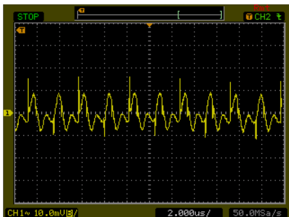
Figure 23: AXA00B18-L Ripple and Noise Measurement Vin = 24Vdc Load: Io = 0.83A Ch 1: Vo
