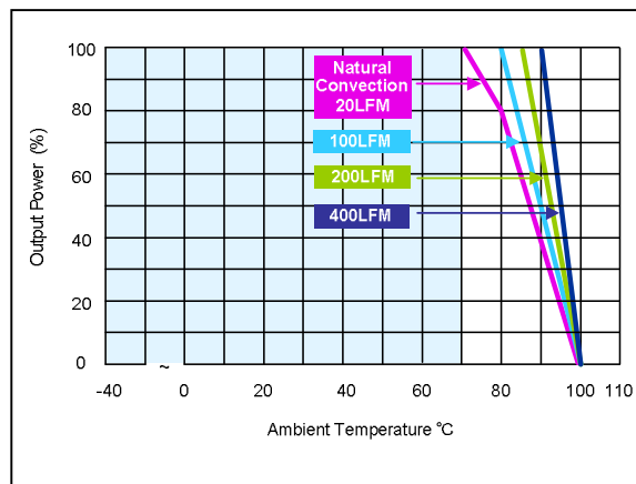
Figure 8: AXA02F18-L Derating Curves (with heatsink) Vin = 24Vdc Load: Io = 0 to 2.2A
