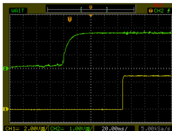
Figure 56: AXA00AA18-L Output Voltage Startup Characteristic by Vin Vin = 24Vdc Load: Io = \pm 1 A Ch1: Vo Ch2: Vin
