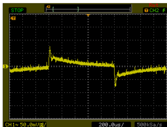
Figure 14: AXA02A18-L Transient Response Vin = 24Vdc Load: Io = 100% to 75% load change Ch 1: Vo
