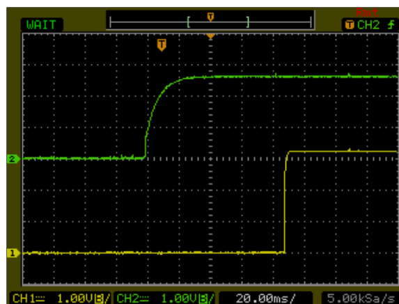
Figure 6: AXA02F18-L Output Voltage Startup Characteristic by Vin Vin = 24Vdc Load: Io = 2.2A Ch1: Vo Ch2: Vin
