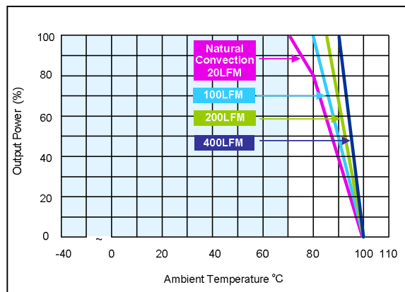
Figure 38: AXA00C18-L Derating Curves (with heatsink) Vin = 24Vdc Load: Io = 0 to 0.67A
