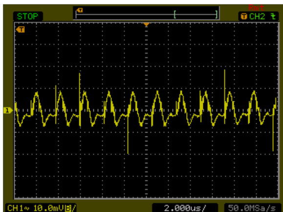
Figure 113 : AXA00C36-L Ripple and Noise Measurement Vin = 48Vdc Load: Io = 0.67A Ch 1: Vo
