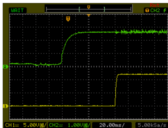
Figure 146: AXA000BB36-L Output Voltage Startup Characteristic by Vin Vin = 48Vdc Load: Io = \pm 0.41 A Ch1: Vo Ch2: Vin
