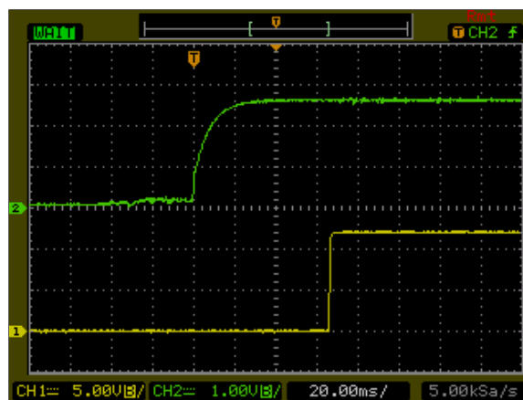
Figure 106: AXA00B36-L Output Voltage Startup Characteristic by Vin Vin = 48Vdc Load: Io = 0.83A Ch1: Vo Ch2: Vin
