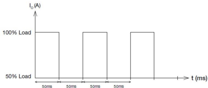
Figure 6. Dynamic Load
