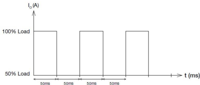
Figure 6. Dynamic Load
