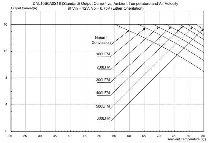
Figure 35: DNL10S0A0S16 (Standard) Output current vs. ambient temperature and air velocity @ Vin=12V, Vo=0.75V(Either Orientation)
