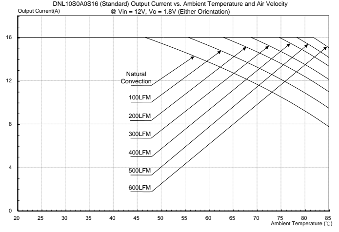
Figure 34: DNL10S0A0S16 (Standard) Output current vs. ambient temperature and air velocity @ Vin=12V, Vo=1.8V(Either Orientation)
