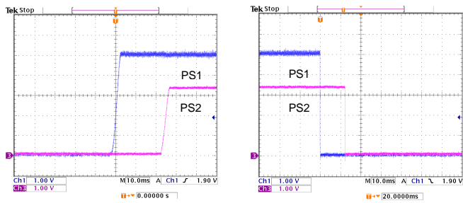
Figure 27: Sequential start-up
