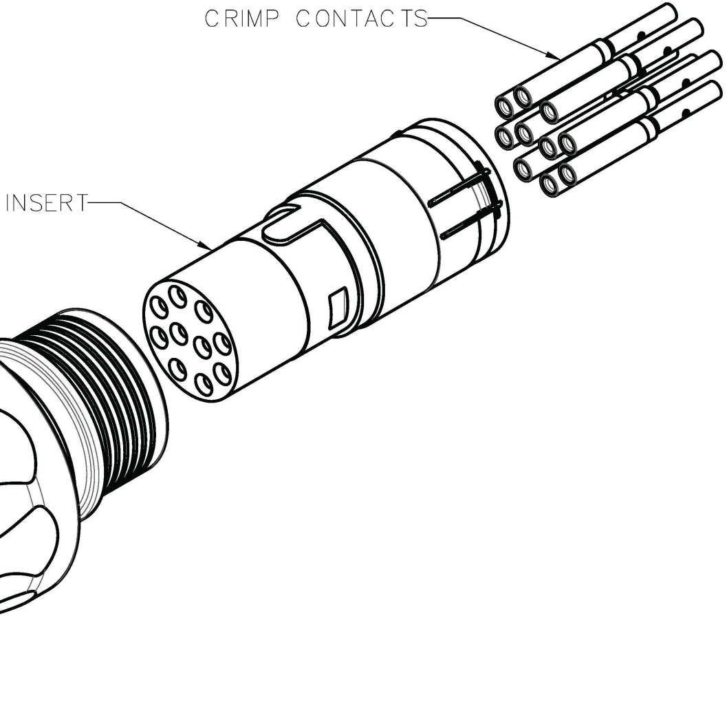
ISOMETRIC VIEW FOR REFERENCE ONLY TMP-B SAN09-010ASC00A SHOWN
