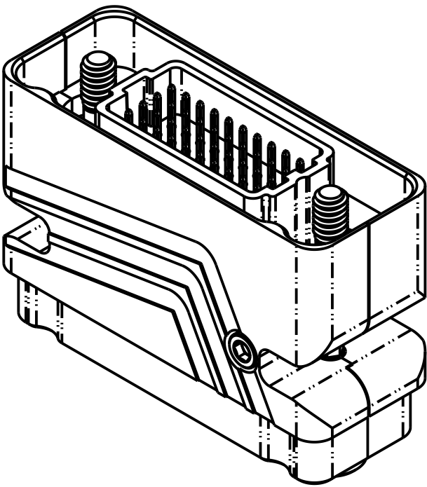
ISOMETRIC VIEW FOR REFERENCE ONLY (PART NUMBER VRCS-04-10-MJFN SHOWN)
