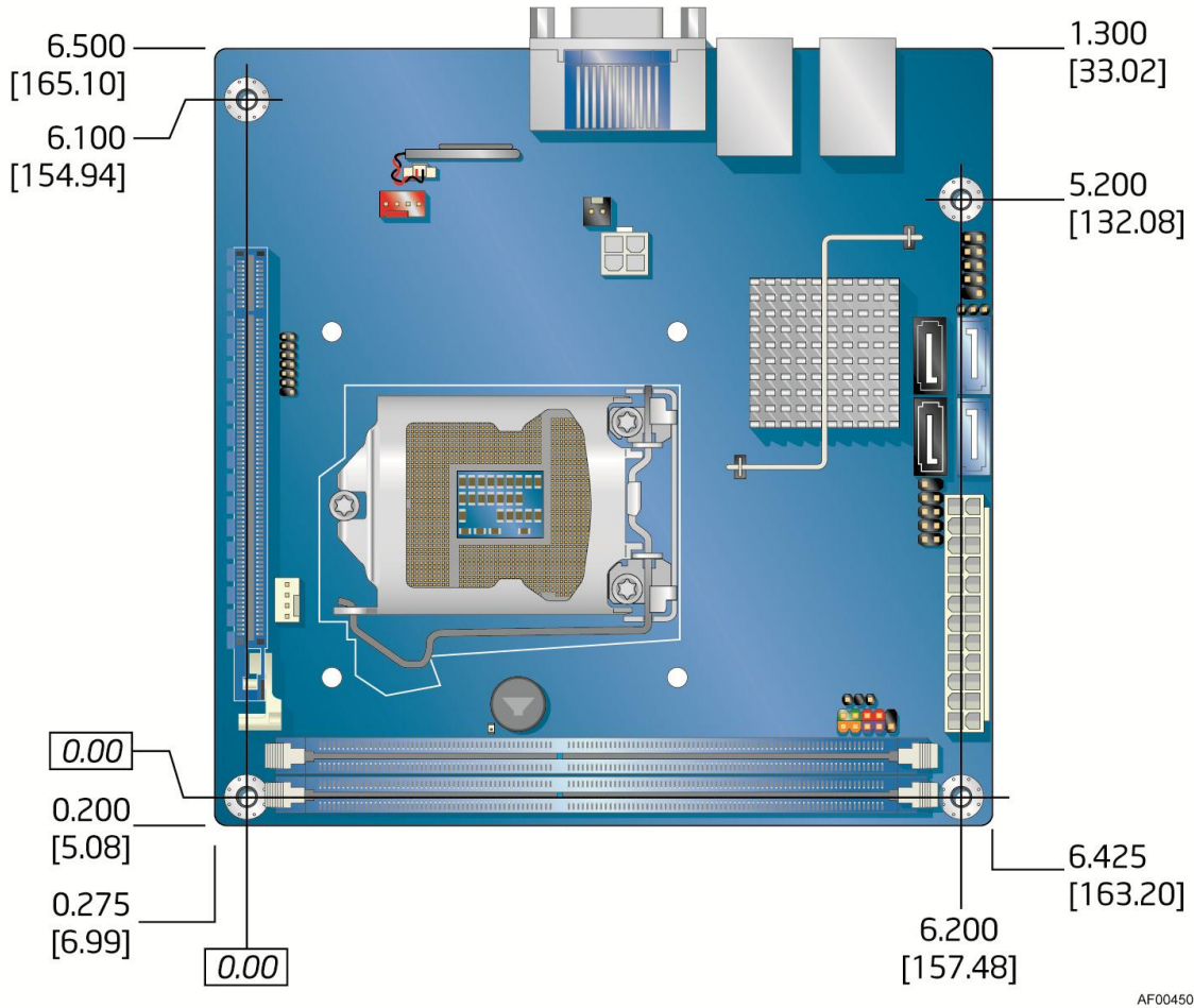
Figure 13. Board Dimensions
