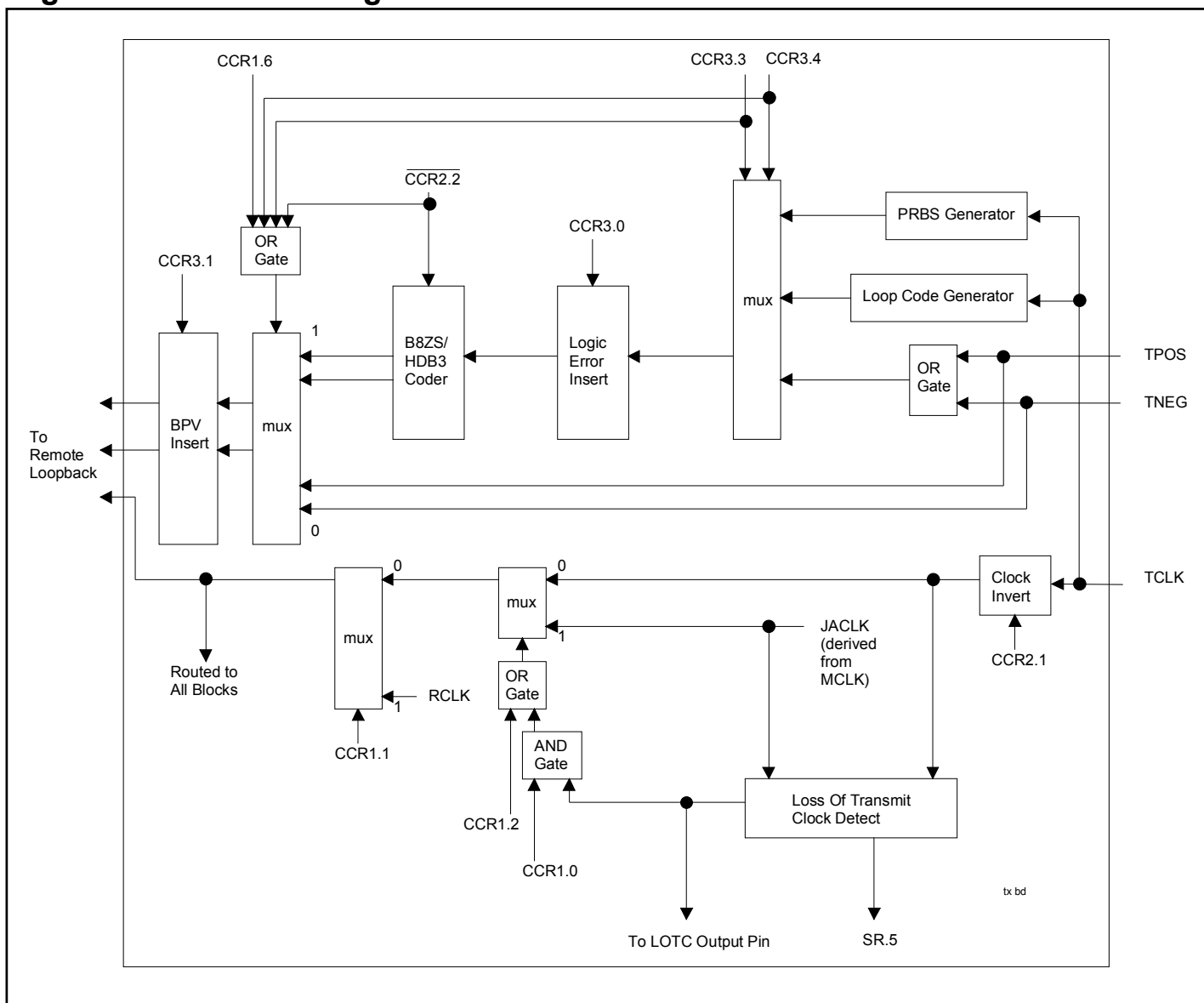
Figure 1-3. Transmit Logic
