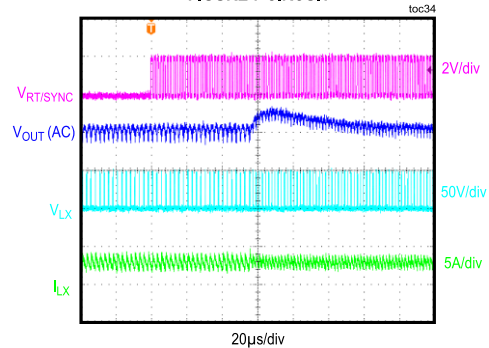
EXTERNAL CLOCK SYNCHRONIZATION FIGURE 7 CIRCUIT
