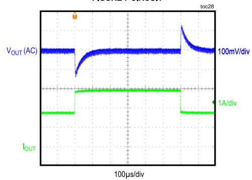
LOAD CURRENT STEPPED FROM 1.8A TO 3A FIGURE 7 CIRCUIT
