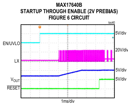
CONDITIONS: FIXED 5V OUTPUT, NO LOAD, PFM MODE
