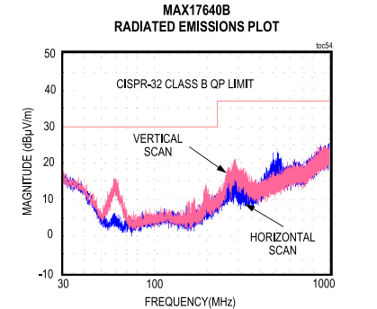
CONDITIONS: V_{IN} = 24V , V_{OUT} = 5V , I_{OUT} = 0.4A MEASURED ON MAX17640BEVKIT#
