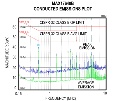
CONDITIONS: V_{IN} = 24V , V_{OUT} = 5V , I_{OUT} = 0.4A MEASURED ON THE MAX17640BEVKIT# WITH L201 = 22µH, C202 = C204 = 1µF/100V/X7R/1206
