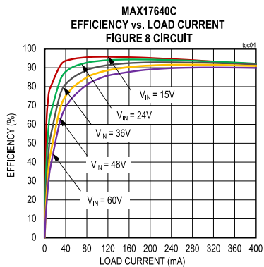
CONDITIONS: ADJUSTABLE 12V OUTPUT, PWM MODE
