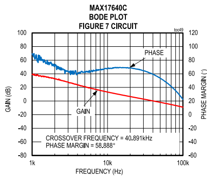
CONDITIONS: ADJUSTABLE 2.5V OUTPUT, 400mA LOAD, PWM MODE
