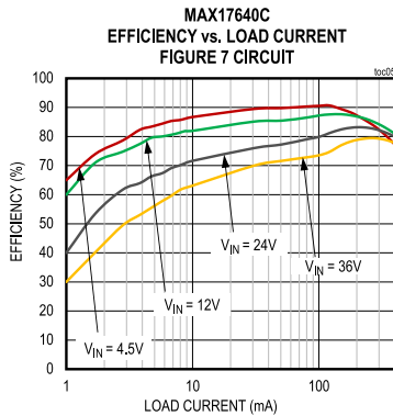
CONDITIONS: ADJUSTABLE 2.5V OUTPUT, PFM MODE
