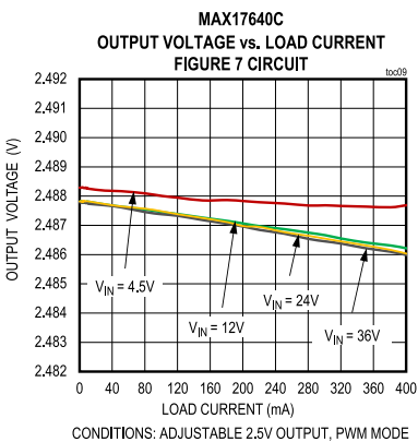
CONDITIONS: ADJUSTABLE 2.5V OUTPUT, PWM MODE
