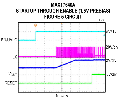
CONDITIONS: FIXED 3.3V OUTPUT, NO LOAD, PFM MODE
