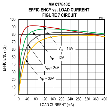
CONDITIONS: ADJUSTABLE 2.5V OUTPUT, PWM MODE
