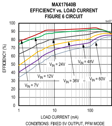
CONDITIONS: FIXED 5V OUTPUT, PFM MODE
