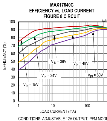
CONDITIONS: ADJUSTABLE 12V OUTPUT, PFM MODE
