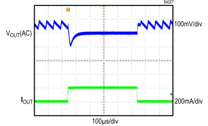
MAX17640A LOAD TRANSIENT RESPONSE FIGURE 5 CIRCUIT
