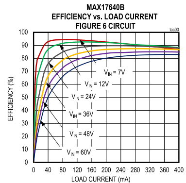
CONDITIONS: FIXED 5V OUTPUT, PWM MODE
