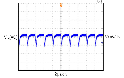
MAX17640C INPUT VOLTAGE RIPPLE FIGURE 7 CIRCUIT
