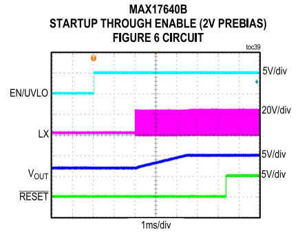
CONDITIONS: FIXED 5V OUTPUT, 400mA LOAD, PWM MODE
