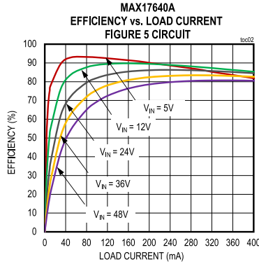
CONDITIONS: FIXED 3.3V OUTPUT, PWM MODE
