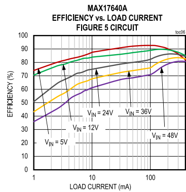
CONDITIONS: FIXED 3.3V OUTPUT, PFM MODE
