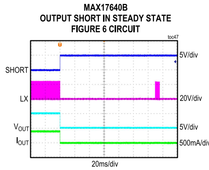
CONDITIONS: FIXED 5V OUTPUT, 400mA LOAD, PWM MODE
