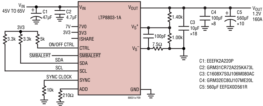
Figure 9. 1.2V 160A 600kHz Step-Down μModule with PMBus
