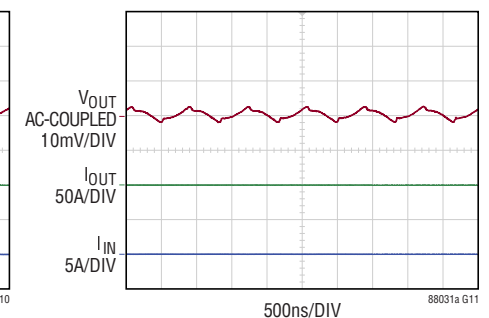
65V IN No Load V OUT Ripple
