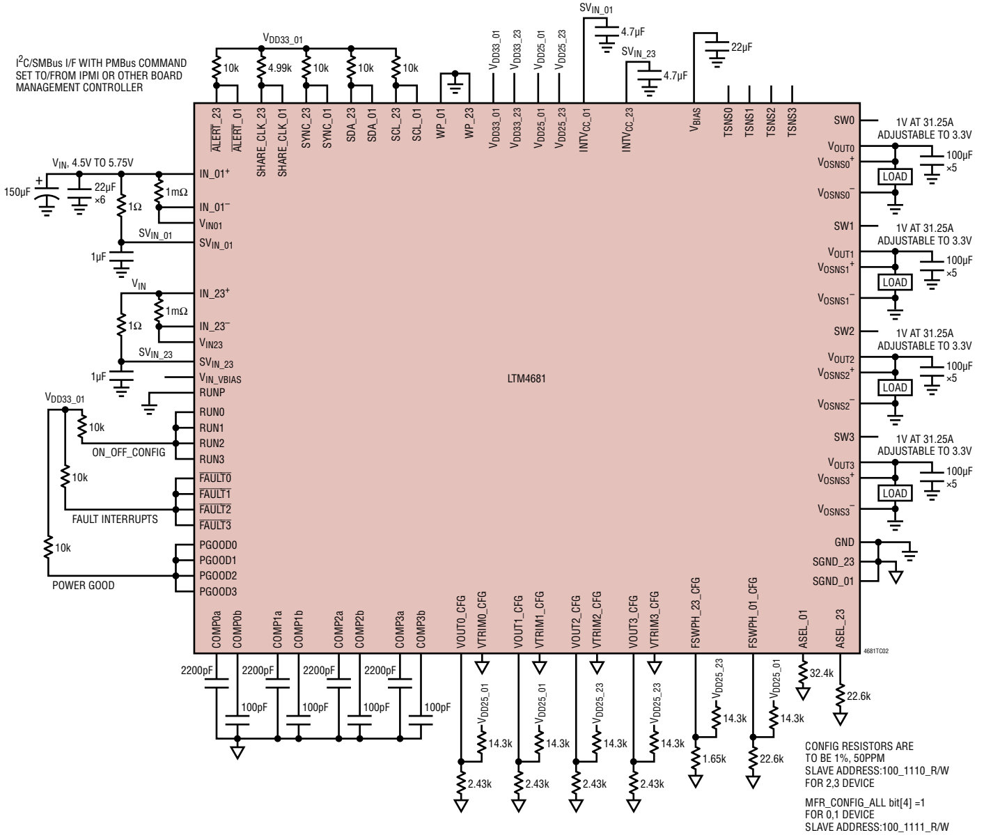
Test Circuit 2.
