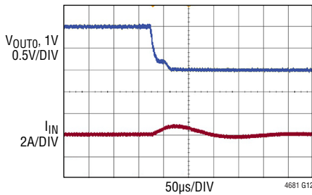
FIGURE 48 CIRCUIT, 12\text{V}_{\text{IN}} , NO LOAD ON \text{V}_{\text{OUT0}} PRIOR TO APPLICATION OF SHORT-CIRCUIT USE HIGH RANGE OF I LIMIT SYSTEM SHORT-CIRCUIT USING LOW IMPEDANCE COPPER ACROSS OUTPUT (HARD SHORT)
