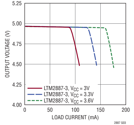
V_{CC2} or V_{L2} Output Voltage vs Input Voltage and Load Current
