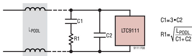
Figure 8. Snubber Network
