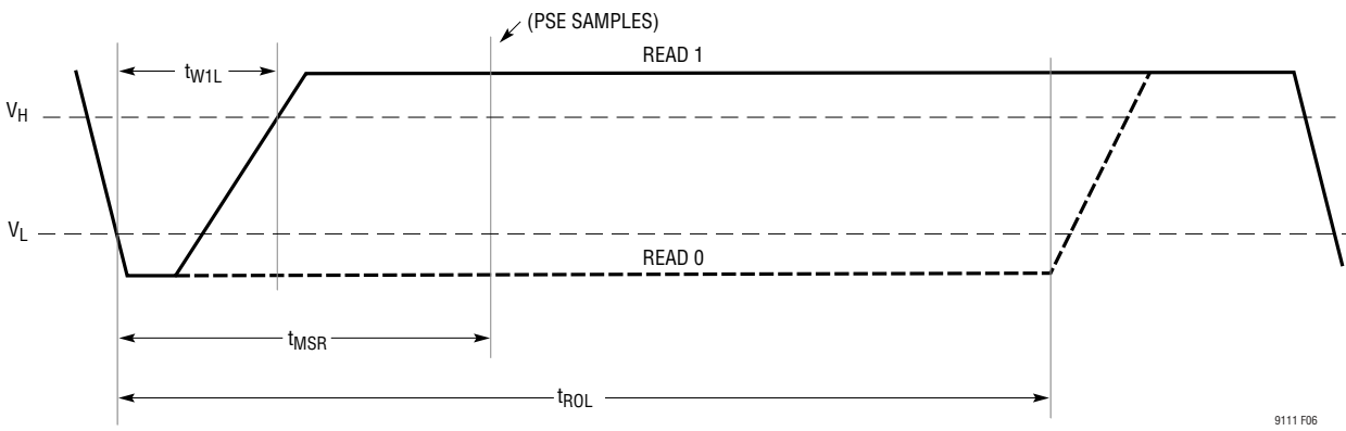
Figure 6. SCCP Read Slot
