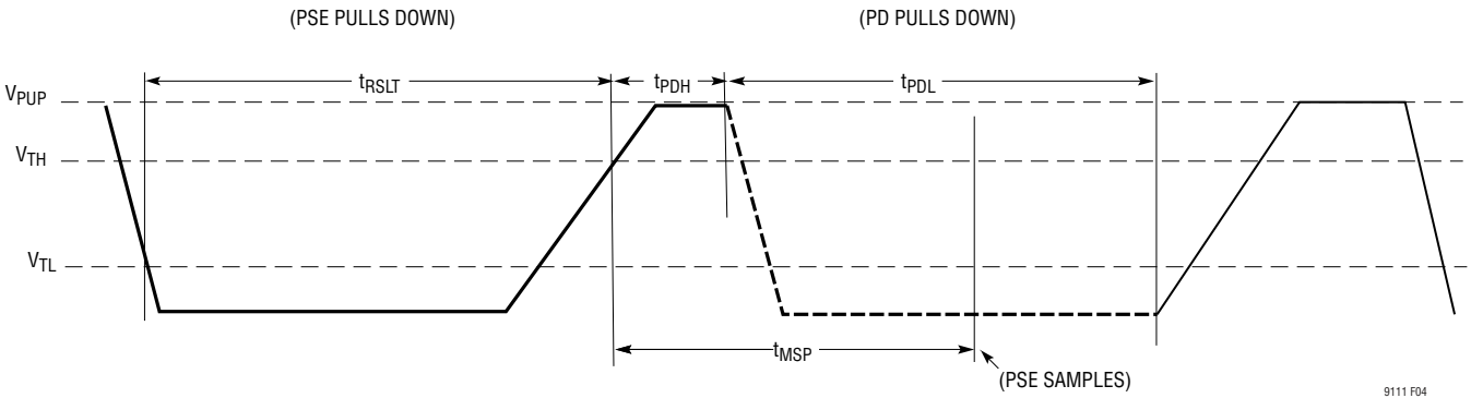
Figure 4. SCCP Initialization
