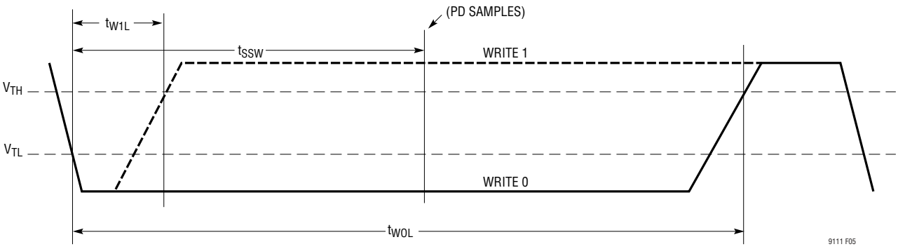
Figure 5. SCCP Write Slot
