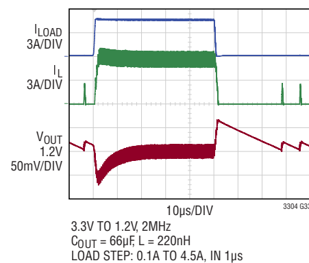
Load Transient Response, Burst Mode Operation
