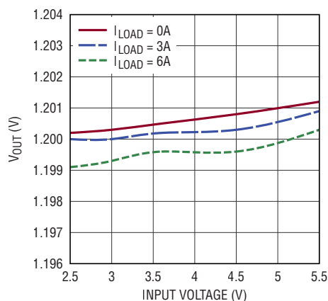
V_{OUT} Line Regulation, V_{OUT} = 1.2V Application, Forced Continuous Mode
