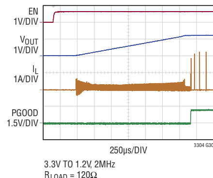
Start-Up Waveforms, Burst Mode Operation
