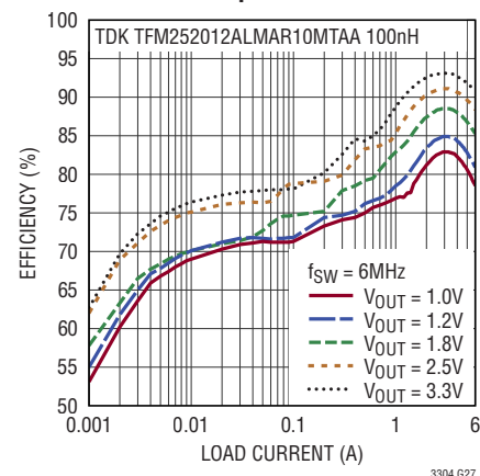
Efficiency, V_{IN} = 5V , Burst Mode Operation
