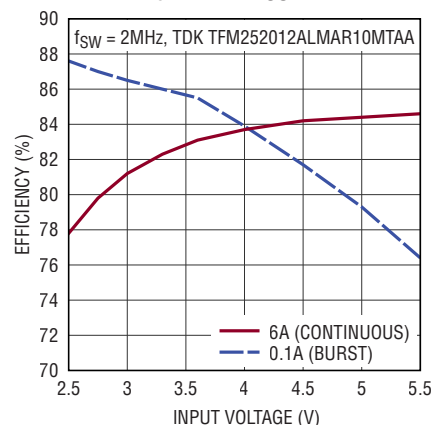
Efficiency vs V_{IN} , V_{OUT} = 1.2V
