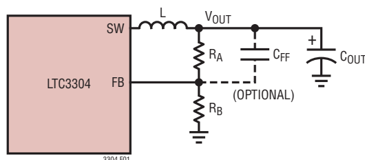
Figure 1. Feedback Resistor Network for the LTC3304 Adjustable Version
