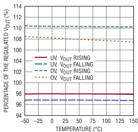
UV, OV PGGOOD Thresholds vs Temperature
