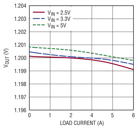
V_{OUT} Load Regulation, V_{OUT} = 1.2V Application, Forced Continuous Mode
