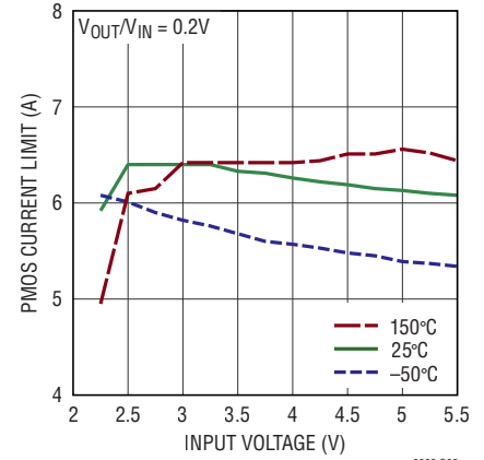
PMOS Current Limit vs V_{IN}
