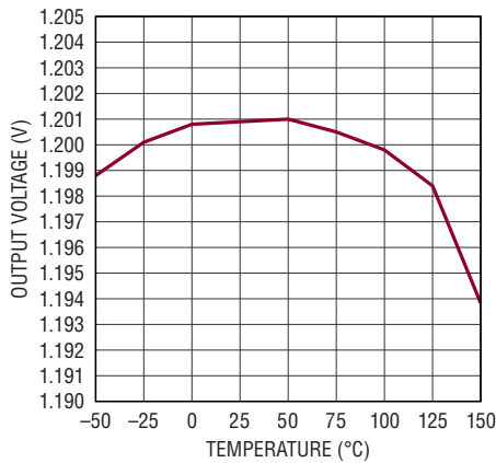
Normalized Regulation Voltage (to 1.2V) vs Temperature
