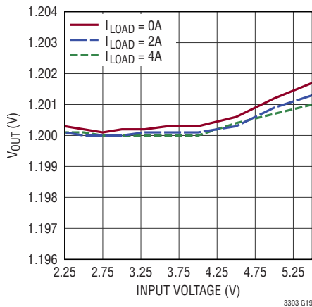
V_{OUT} Line Regulation, V_{OUT} = 1.2V Application, Forced Continuous Mode
